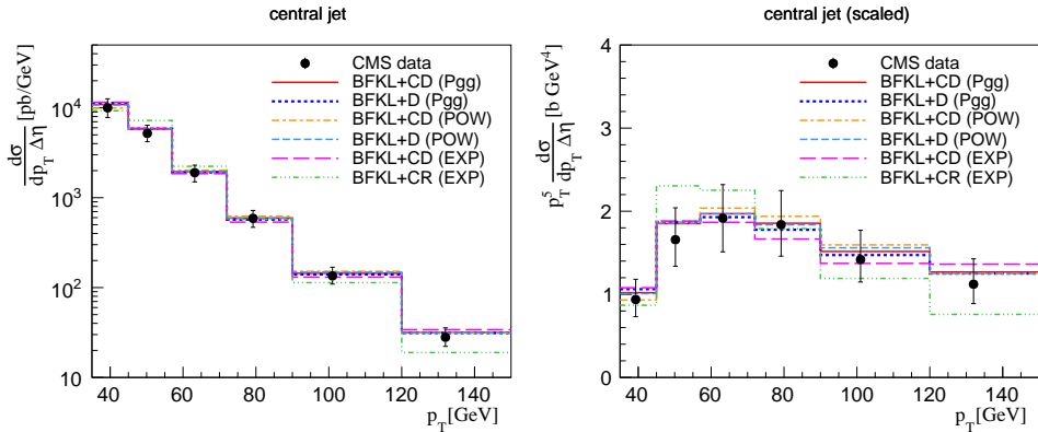
Fig. 2. The p_T spectra of the central jet calculated using the best fits for individual models versus the CMS data. For the right plot, the cross sections have been scaled by p_T^5 to better see the differences between the models.
