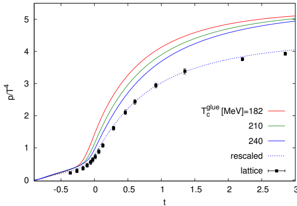
Fig. 2. (Color online) The normalized pressure as a function of the reduced temperature (see the text for the dashed/blue curve).
