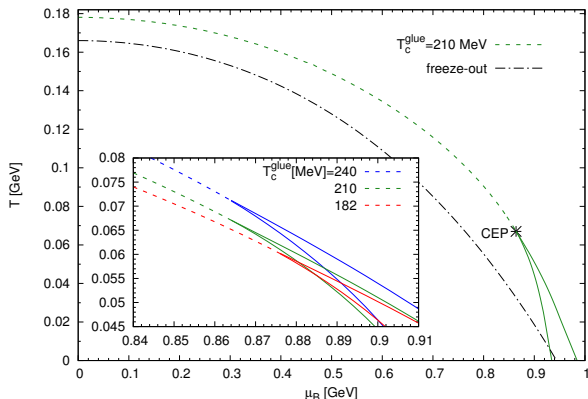
Fig. 4. The phase diagram obtained with T_c^{\text{glue}} = 210 MeV. The inset shows the influence of the T_c^{\text{glue}} on the location of the CEP.
