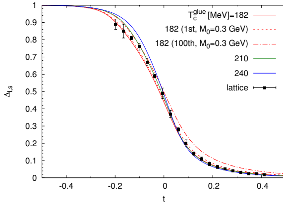
Fig. 1. The subtracted chiral condensate \Delta_{l,s} at \mu_B = 0 as a function of the reduced temperature t = T/T_c - 1 .
