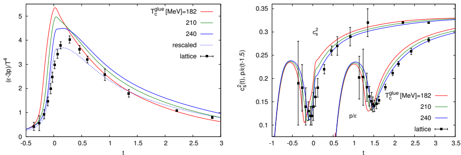
Fig. 3. The interaction measure (left panel) and the square of the speed of sound c_s^2 and the appropriately shifted ratio of the pressure to the energy density p/\epsilon (right panel) as a function of t = T/T_c - 1 for three values of T_c^{\text{glue}} .
