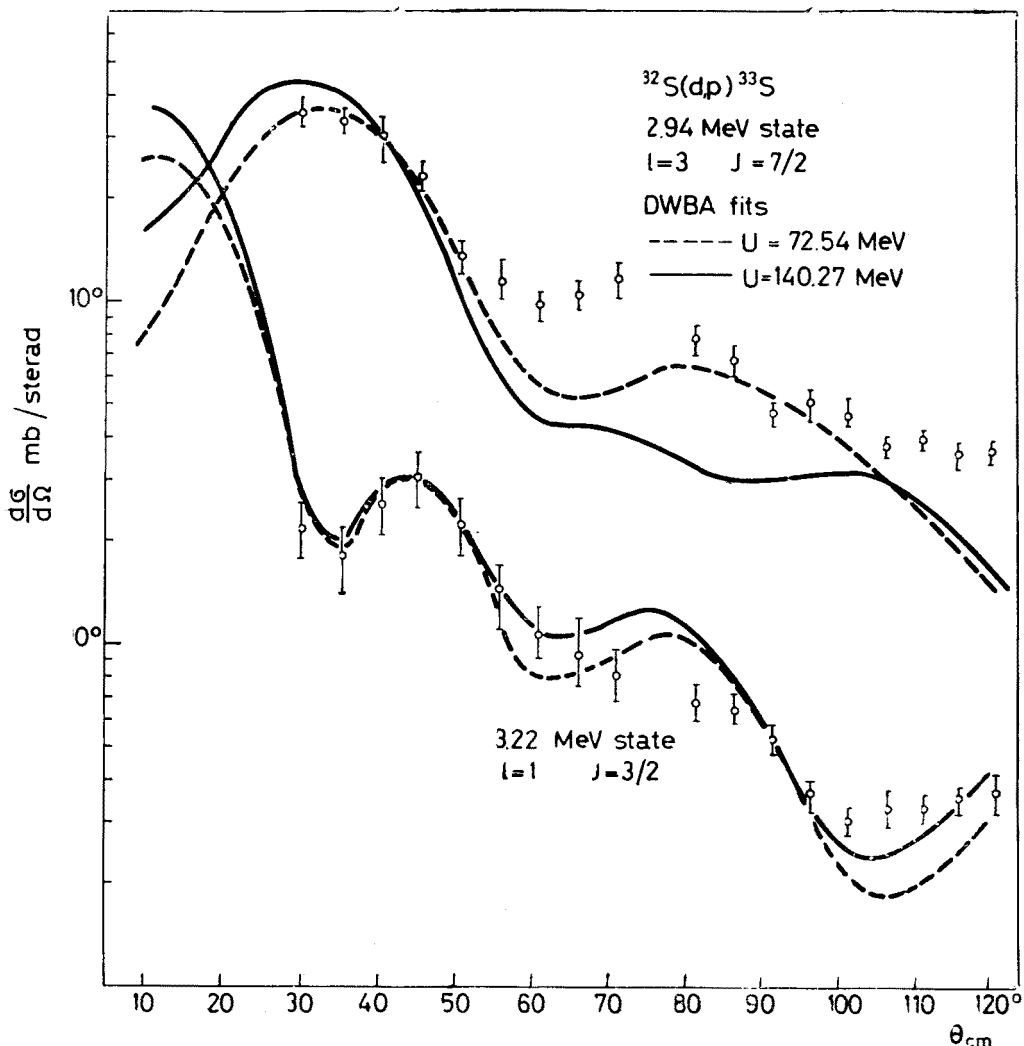
Fig. 6. Angular distributions for the 2.94 MeV and 3.22 MeV state transitions in the ^{32}\text{S}(\text{d}, \text{p})^{33}\text{S} reaction. The curves represent the DWBA calculations with two sets of deuteron optical model parameters
