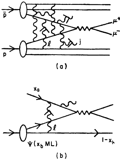
Fig. 2. (a) Representation of initial state interactions in perturbative QCD. (b) Simplest example of induced radiation by initial state interactions in q\pi \rightarrow l\bar{l}X . Two different physical radiation processes are included in this Feynman amplitude depending on whether the intermediate state before or after the gluon emission is on-shell. The two bremsstrahlung processes destructively interfere at energies large compared to a scale proportional to the target length L .
