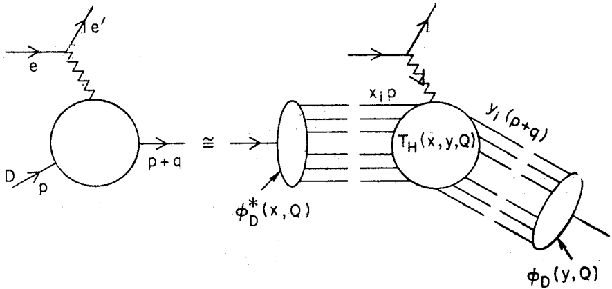
Fig. 10. Factorization of the deuteron form factor at large Q^2
