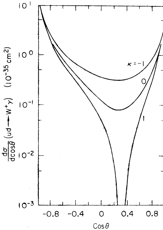
Fig. 6. The differential cross-section for u\bar{d} \rightarrow W^+\gamma for SU(2) \times U(1) gauge theory in Born approximation. The subprocess cross section vanishes identically near \cos \theta^{\gamma d} = 1/3
