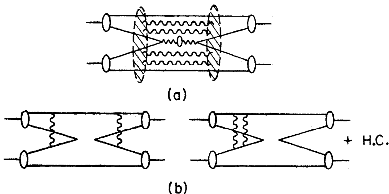
Fig. 3. (a) Representation of initial state interactions in the Drell-Yan cross section d\sigma/dQ^2 dx . (b) Example of two-loop initial state interactions which cancel by unitarity in an Abelian gauge theory. In QCD these two contributions have different color factors
