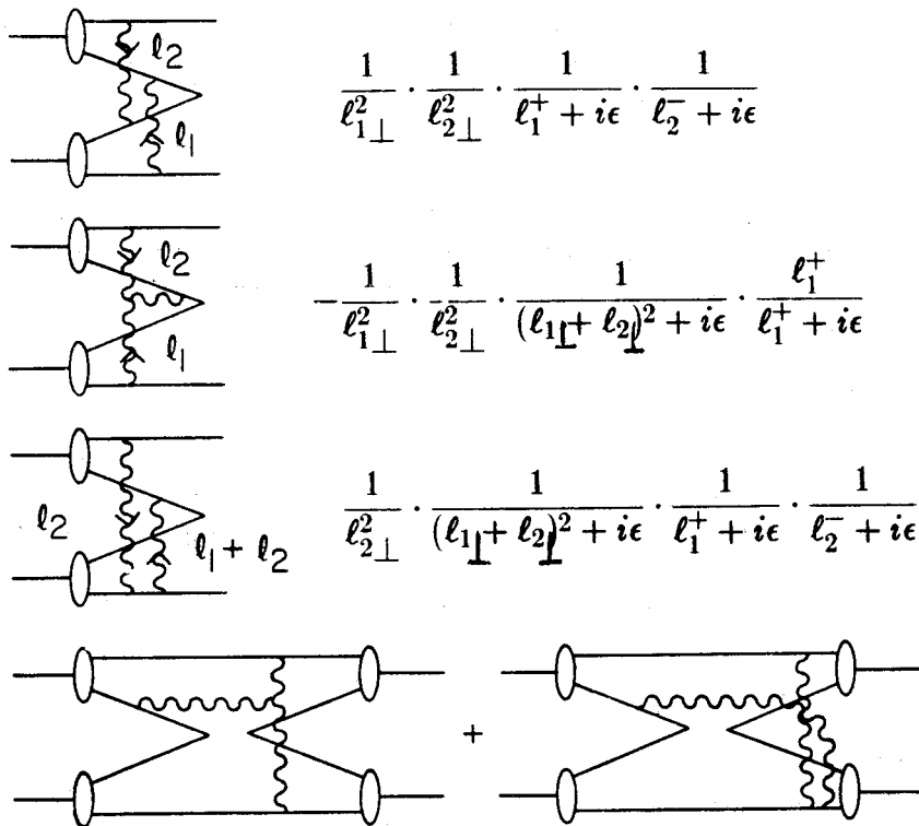
Fig. 4. Representative active spectator initial state interactions for \pi\pi \rightarrow \bar{u}X in QCD involving C_F C_A evaluated in Feynman gauge. The real part of the two loop contributions represented by (a), (b), (c) (including mirror diagrams) vanishes at high energies. The imaginary parts cancel against the gluon emission contribution represented in (d) and (e)
