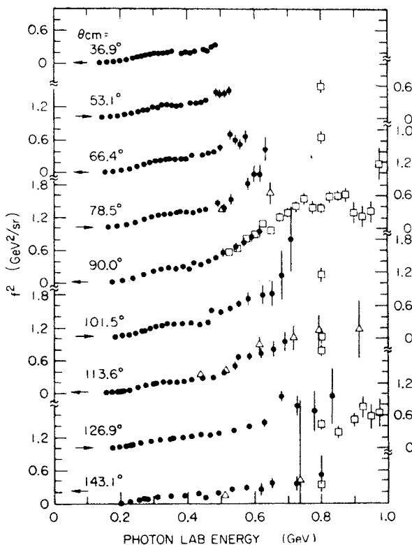
Fig. 13. Comparison of deuteron photodisintegration data [66] with the scaling prediction (35) which requires f^2(\theta_{CM}) to be independent of energy at large momentum transfer
