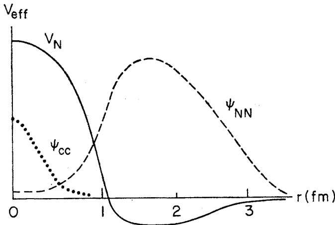
Fig. 12. Schematic representation of the deuteron wavefunction in QCD indicating the presence of hidden color six-quark components at short distances
