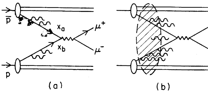
Fig. 1. (a) Gluon emission associated with QCD evolution of structure functions for the Drell-Yan process, p\bar{p} \rightarrow \mu^+\mu^-X . (b) Gluon emission associated with initial state interactions for the Drell-Yan process.
