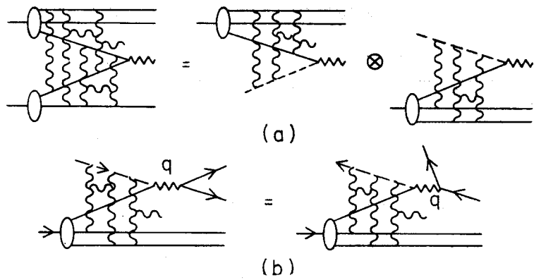
Fig. 5. (a) Schematic of the general decomposition required to prove weak factorization to general orders in QCD. The dotted line corresponds to the eikonal line integral of Eq. (10). Vertex corrections which modify the hard scattering amplitude are not shown. These provide a separate factor on the right hand side of 7(a). (b) The relationship between Drell-Yan and deep inelastic lepton scattering eikonal-extended structure functions required to prove factorization
