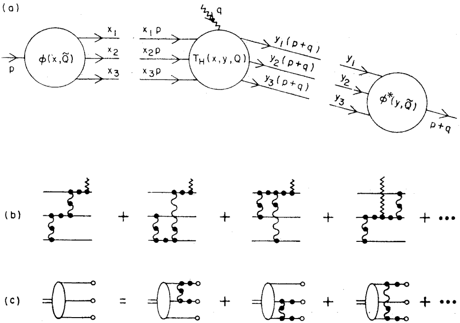
Fig. 8. (a) Factorization of the nucleon form factor at large Q^2 in QCD. The optimal scale \tilde{Q} for the distribution amplitude \phi(x, \tilde{Q}) is discussed in reference [50]. (b) The leading order diagrams for the hard scattering amplitude T_H . The dots indicate insertions which enter the renormalization of the coupling constant. (c) The leading order diagrams which determine the Q^2 dependence of \phi_B(x, Q)
