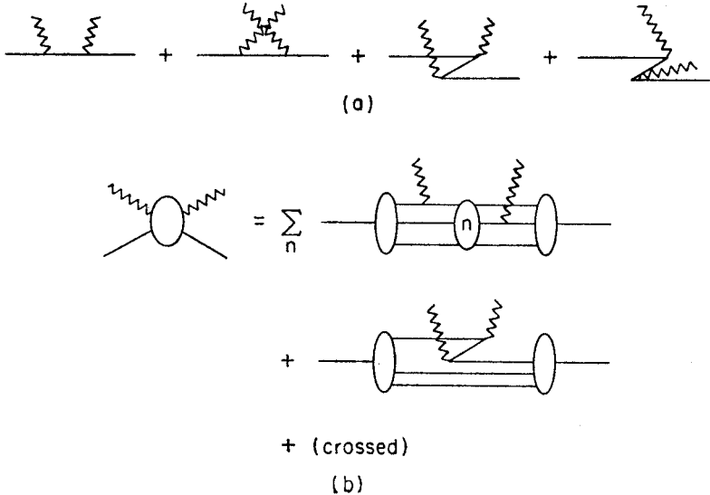
Fig. 15. Time-ordered contributions to (a) The Compton amplitudes in a local Lagrangian theory such as QED. Only the Z-graphs contribute in the forward low energy limit. (b) Calculation of the Compton amplitude for composite systems
