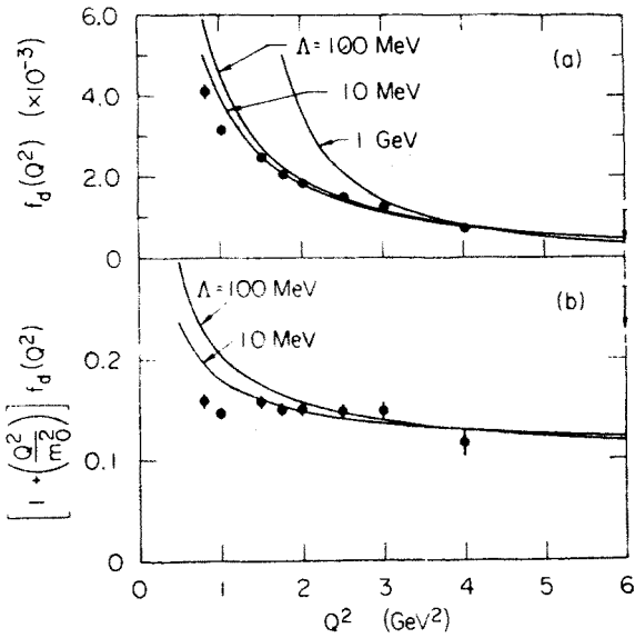
Fig. 11. (a) Comparison of the asymptotic QCD prediction (31) with experiment (16) using F_N(Q^2) = (1 + Q^2/0.71 \text{ GeV}^2)^{-2} . The normalization is fit at Q^2 = 4 \text{ GeV}^2 . (b) Comparison of the prediction [1 + (Q^2/m_0^2)]f_d(Q^2) \propto (\ln Q^2)^{-1-2/5C_F/\beta} with data. The value m_0^2 = 0.28 \text{ GeV}^2 is used
