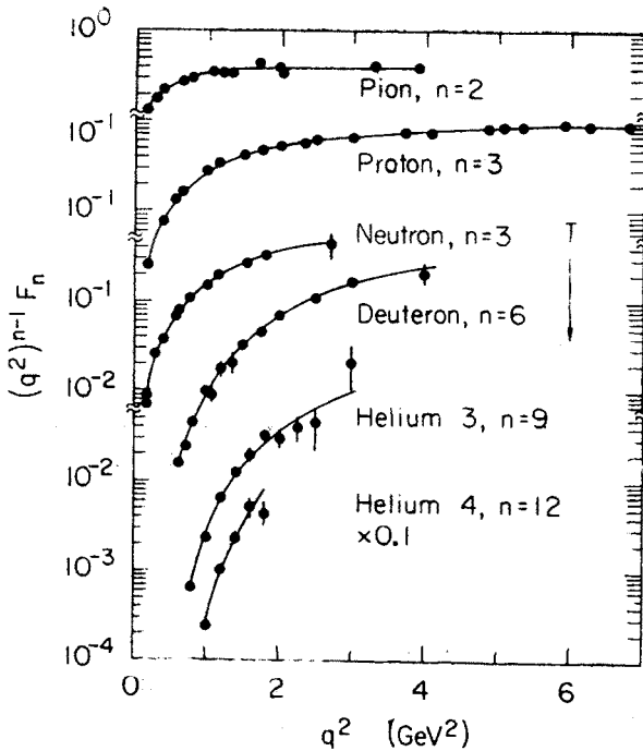
Fig. 9. Comparison of experiment with the QCD dimensional counting rule (Q^2)^{n-1}F(Q^2) \sim \text{const} for form factors. The proton data extends beyond 30 \text{ GeV}^2 (see reference [58])
