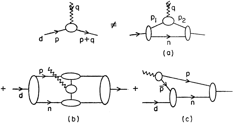
Fig. 14. Critique of the standard nuclear physics approach to the deuteron form factor at large Q^2 . (a) The effective nucleon form factor has one or both legs off shell: |p_1^2 - p_2^2| \sim q^2/2 . (b) Meson exchange currents are suppressed in QCD because of off shell form factors. (c) The nucleon pair contribution is suppressed because of nucleon compositeness. Contact terms appear only at the quark level
