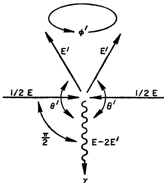
Fig. 7. Kinematics for the null zone for e^-e^- \rightarrow e^-e^-\gamma
