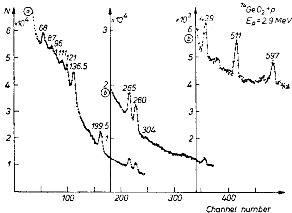
Fig. 3. Spectrum of gamma radiation emitted from ^{74}\text{GeO}_2 target bombarded with 2.9 MeV protons
