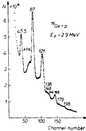
Fig. 5. Spectrum of gamma radiation emitted from ^{76}\text{Ge} target bombarded with 2.9 MeV protons
