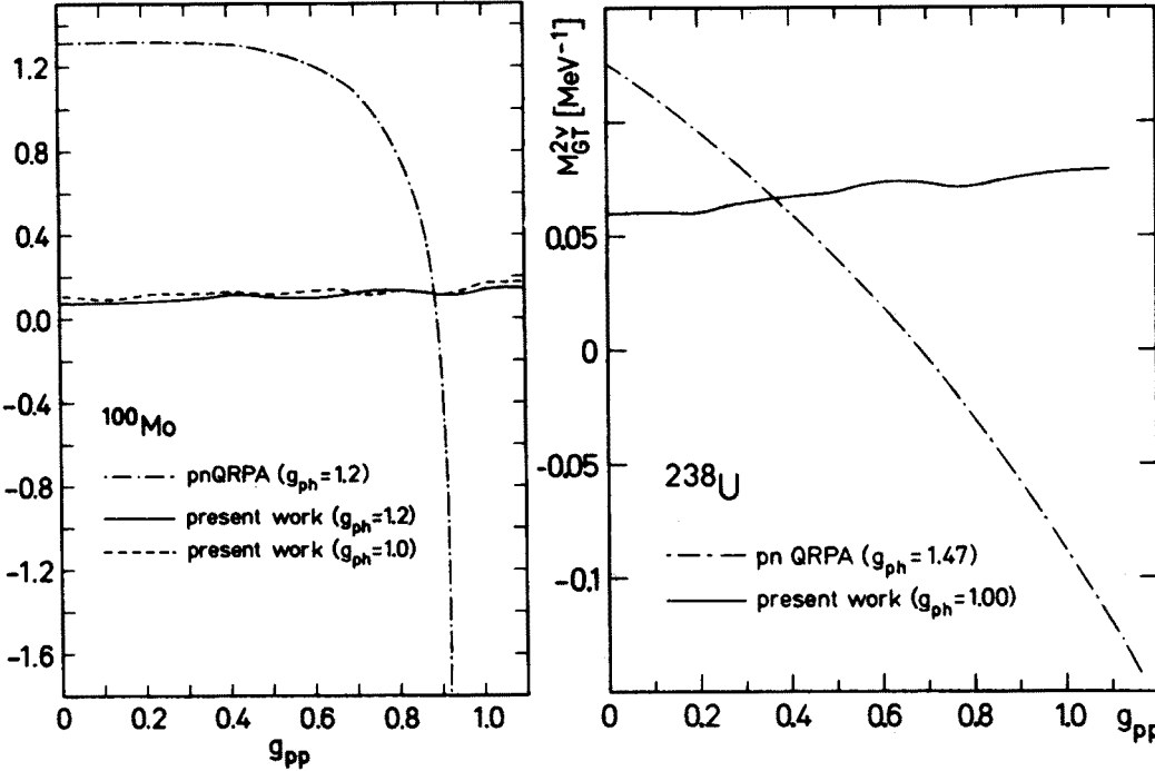
Figure 12: The matrix elements M_{GT}^{2\nu} of \beta\beta_{2\nu} decay of ^{100}\text{Mo} and ^{238}\text{U} as function of g_{pp} in QRPA and in OEM (from [wu91,wu92b])
