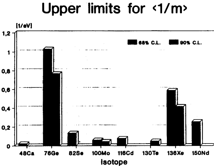
Figure 16: Neutrino mass limits deduced from \beta\beta_{0\nu} detector experiments (i. e. not including geochemical experiments)
