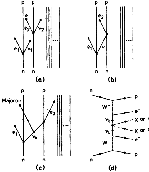
Figure 8: Graphs for \beta\beta_{2\nu} , \beta\beta_{0\nu} , \beta\beta_{0\nu\chi} and \beta\beta_{0\nu2\chi} decay
