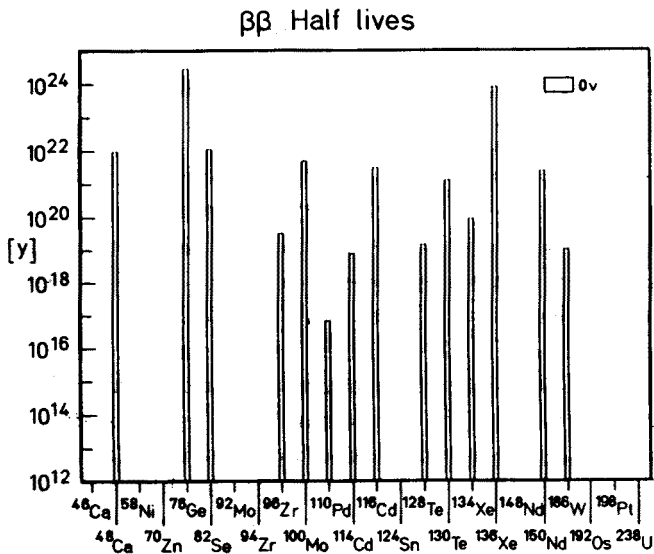
Figure 15: Measured \beta\beta_{0\nu} half-life limits
