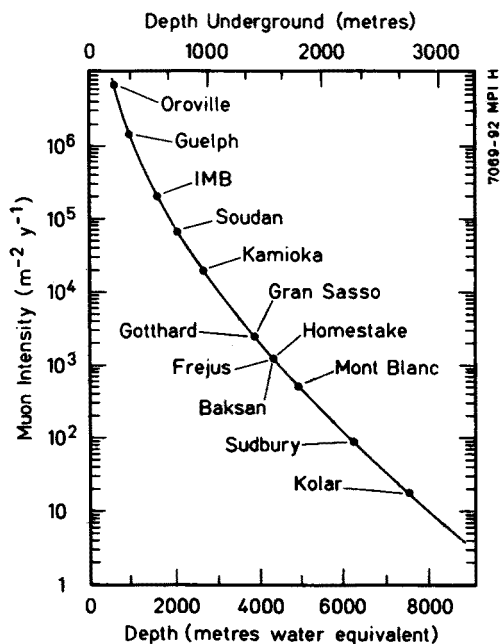
Figure 14: Some of the main underground laboratories, in which double beta decay experiments are performed, and their depth (in meter water equivalent) and reduction of cosmic radiation induced muon flux
