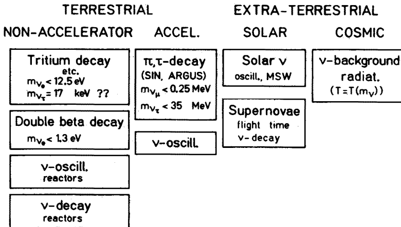
Figure 2: Classification of experiments investigating the neutrino mass
