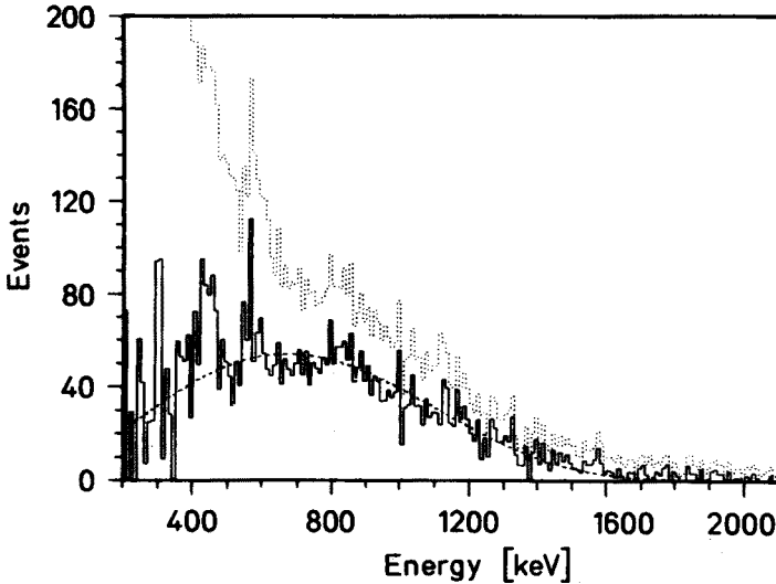
Figure 21: Comparison of the 527 kg-d measured spectrum (dotted curve, lines cut out) and after the subtraction described in the text (solid curve). Also shown is a fitted 2\nu -spectrum for T_{1/2}^{2\nu} = 1.42 \cdot 10^{21} y (dashed curve)
