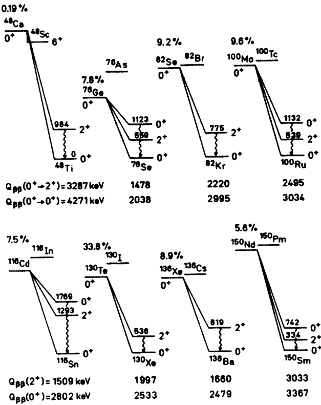
Figure 13: Some of the at present most studied \beta\beta emitters
