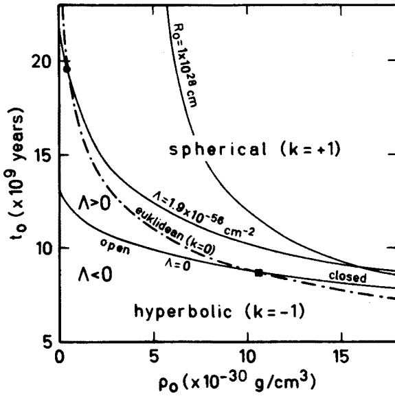
Figure 6: Relation between the age of universe t_0 and present cosmic matter density \rho_0 for various cosmological model types, with cosmological constant \Lambda and metric parameter k as parameters ( H_0 is fixed to 75 km/Mpc·s). In Friedmann-Einstein models ( \Lambda=0 ) t_0 cannot exceed 13 \cdot 10^9 y. Moreover this limiting value would only be obtained in strongly hyperbolic models without dark matter, Euclidean metric would restrict t_0 further to 8.7 Gy. Larger values for t_0 can be obtained in Euclidean models if \Lambda > 0 (from [kla86])
