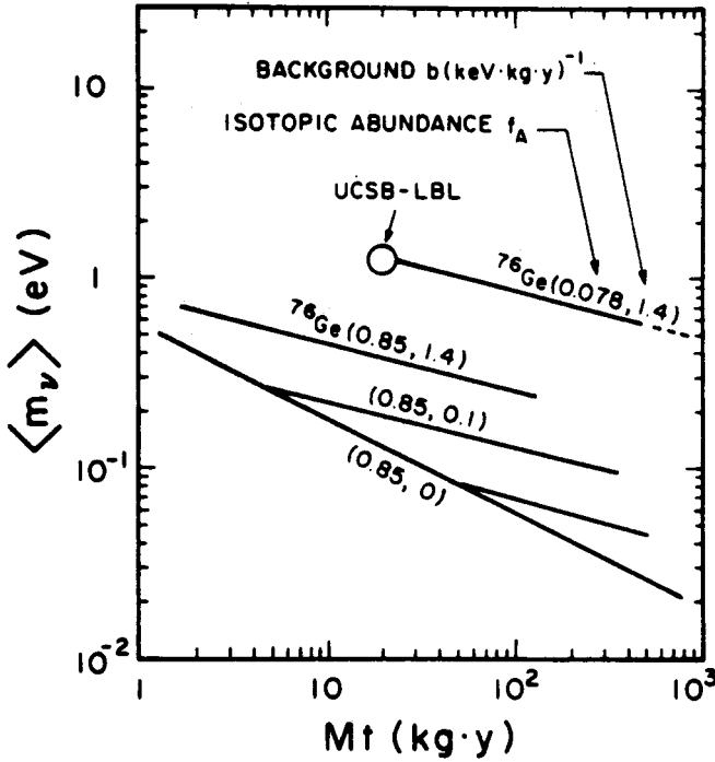
Figure 24: The ranges of neutrino mass which can be probed with Ge-detectors of different enrichment in ^{76}\text{Ge} , as function of the product detector mass times measuring time (kg·y) (from [moe91])
