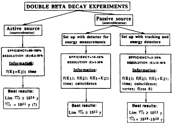
Figure 17: Classification of double beta decay experiments (after [zde92c])
