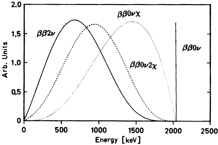
Figure 9: Shapes of the electron sum spectra in the cases of \beta\beta_{2\nu} , \beta\beta_{0\nu} , \beta\beta_{0\nu\chi} and \beta\beta_{0\nu2\chi} decay (for the case of ^{76}\text{Ge} decay)
