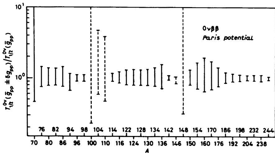
Figure 10: The uncertainty of QRPA-calculated \beta\beta_{0\nu} rates originating from the limited knowledge of the particle-particle force for the potential double beta emitters (from [sta90b])
