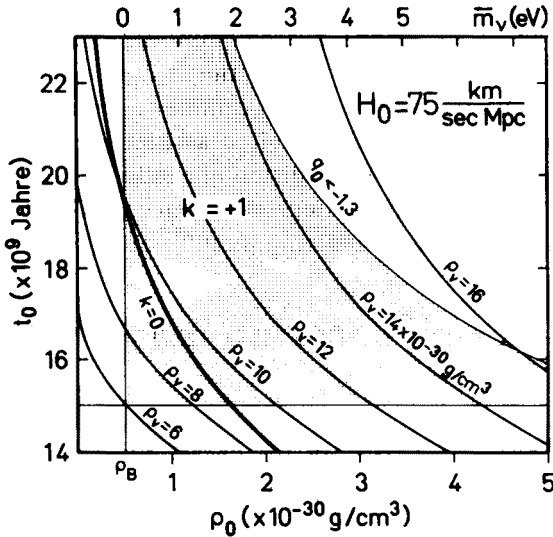
Figure 7: The relation between t_0 and \rho_0 as in Fig. 6, however, the parameter range of interest shown in more detail. The hatched area corresponds to boundary conditions \rho_0 \geq \rho_B , q_0 < -1.3 and t_0 = 15 \text{ Gy} . In this area only models with \rho_V > 0 are allowed. For Euclidean metric ( k=0 ) this holds also for H_0=50 \text{ km/Mpc.s} down to ages t_0 > 13 \text{ Gy} . An upper limit of the neutrino mass can be read from the upper scale, corresponding to attributing the non-baryonic dark matter \rho_D = \rho_0 - \rho_B to neutrinos (from [kla86])
