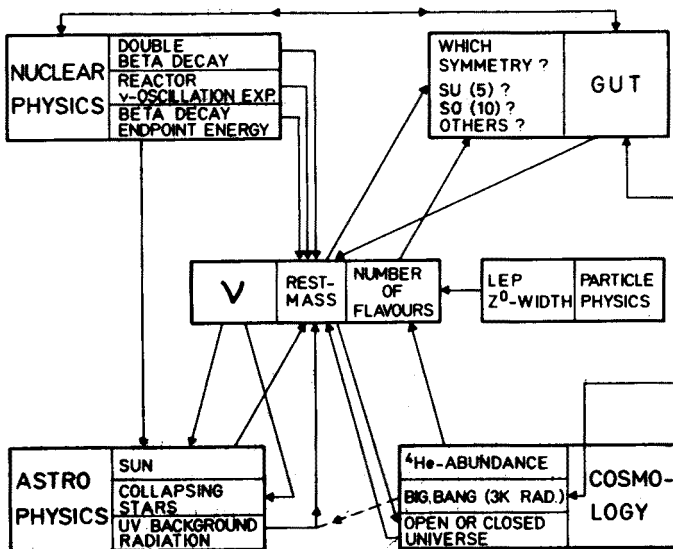
Figure 1: The neutrino and its role in micro- and macrophysics
