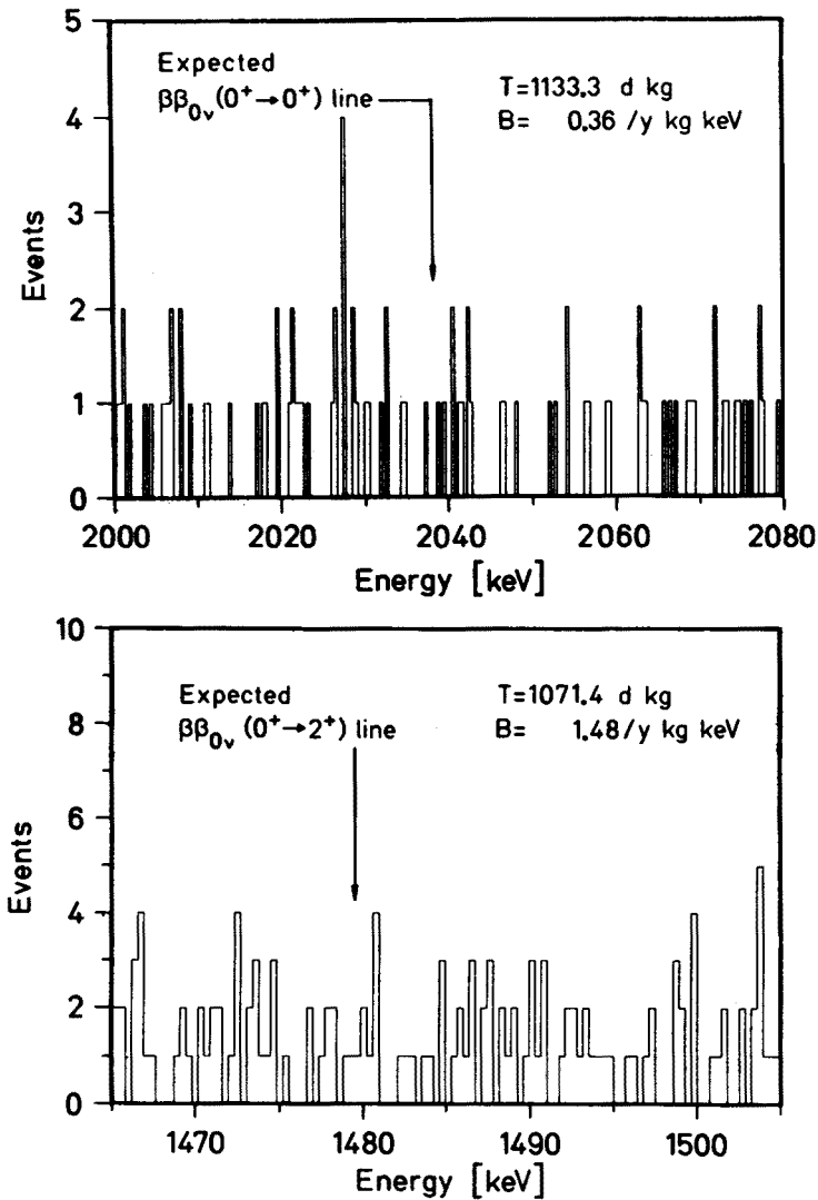
Figure 20: Details of the spectrum of the HEIDELBERG-MOSCOW collaboration in the region of neutrinoless double beta decay to the ground (upper part) and first excited (lower part) state of the daughter nucleus after a measuring time of 1133/1071 kg·d
