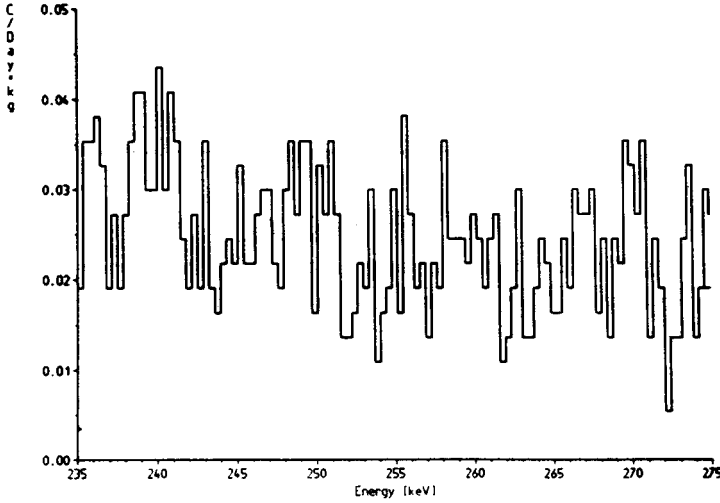
Figure 23: Spectrum measured in 368 kg·d in the range of the 255 keV \gamma -line expected from a decay e^- \rightarrow \gamma + \nu_e
