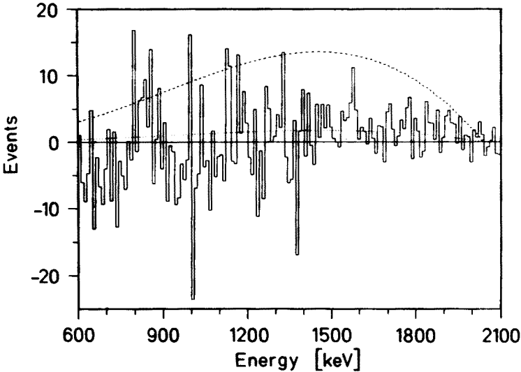
Figure 22: Remaining spectrum after further subtracting from the solid curve in Fig.21 the 2\nu mode, together with a calculated 0\nu\chi spectrum with T_{1/2}^{0\nu\chi} = 3.89 \cdot 10^{22} y (dotted curve). The recently discussed [moe92] coupling constant of 3 \cdot 10^{-4} would yield the dashed curve
