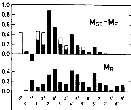
Figure 11: The decomposition of the nuclear matrix element M_{GT}^{0\nu} - M_F^{0\nu} (upper) and M_R (lower) into contributions through intermediate states with spin parity J^\pi for the \beta\beta_{0\nu} decay of ^{76}\text{Ge} \rightarrow ^{76}\text{Se} . In the upper part, the contribution of M_{GT}^{0\nu} and -M_F^{0\nu} are denoted by the filled and open histograms, respectively (from [mut89])
