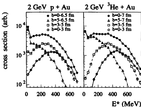
Fig. 2. Excitation energy spectra for 2 GeV p+Au and ^3\text{He} +Au reaction. Intranuclear cascade prediction calculated at thermalization time, t = 30 fm/c. The results for several impact parameter bins.
