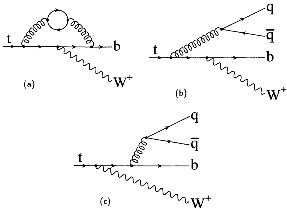
Fig. 1. Diagrams with virtual and real fermions contributing to top's width.
