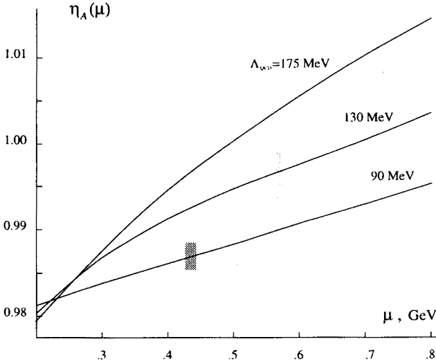
Fig. 3. The value of \eta_A(\mu) for \Lambda_{\overline{\text{MS}}} = 90 \text{ MeV} , 130 \text{ MeV} and 175 \text{ MeV} . The value of \eta_A(\mu) must be used in the QCD-based calculations of the exclusive zero-recoil B \rightarrow D^* form factor when nonperturbative effects are addressed. The shaded bars show the perturbative uncertainty irreducible without considering 1/m_c^3 and 1/m_c^4 effects; they give the lower bound for the corresponding actual nonperturbative corrections.
