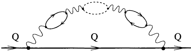
Fig. 2. Perturbative diagrams leading to the IR renormalon uncertainty in m_Q^{\text{pole}} of the order of \Lambda_{\text{QCD}} . The contribution of the gluon momenta below m_Q expresses the classical Coulomb self-energy of the colored particle. The number of bubble insertions into the gluon propagator can be arbitrary.
