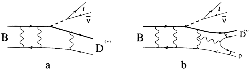
Fig. 1. Exclusive B \rightarrow D^{(*)} (a) and generic (b) semileptonic decays.
