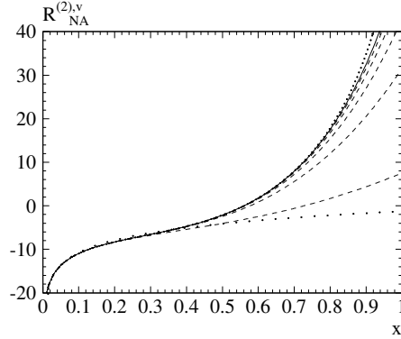
Fig. 2. Non-abelian contribution to R_{\text{had}} as an example for the application of the Large Momentum Procedure [16], plotted over x = 2m/\sqrt{s} . Narrow dots: semi-analytical result from [17], other lines: power corrections up to (m^2/s)^n , n = 0, \dots, 6 .
