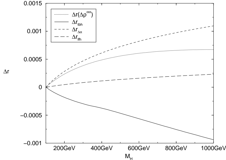
Fig. 1. Higgs-mass dependent fermionic contributions to \Delta r at two-loop order. The different curves show the contribution from the diagrams involving the top/bottom doublet ( \Delta r_{\text{tbh}} ), the contribution proportional to \Delta\alpha ( \Delta r_{\Delta\alpha} ), the contribution of the light fermions ( \Delta r_{\text{lfh}} ), and the approximation of the top/bottom correction by the leading term proportional to m_t^4 ( \Delta r(\Delta\rho^{\alpha\alpha}) ).
