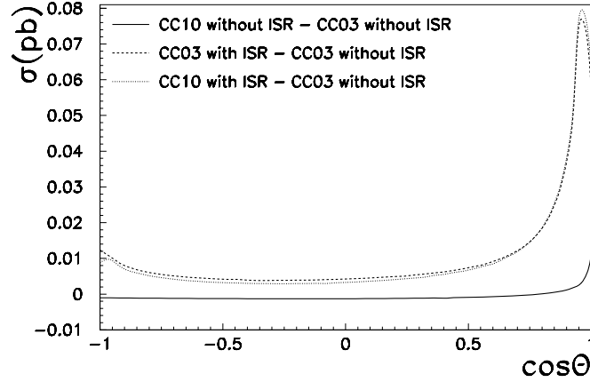
Fig. 1. Differences between Born cross-section and cross-section with initial state radiation.
