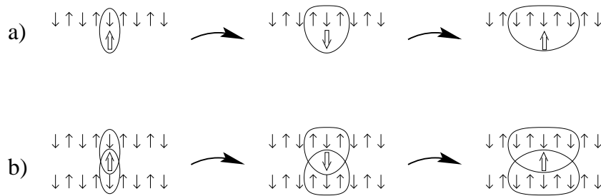
Fig. 1. Sketch of the renormalization group for a) the single-channel Kondo model (local moment compensation) and b) the two-channel Kondo model (local moment over-compensation). Small arrows denote conduction electron spins 1/2 , a heavy arrow a localized spin 1/2 . The curved arrows indicate successive renormalization steps.
