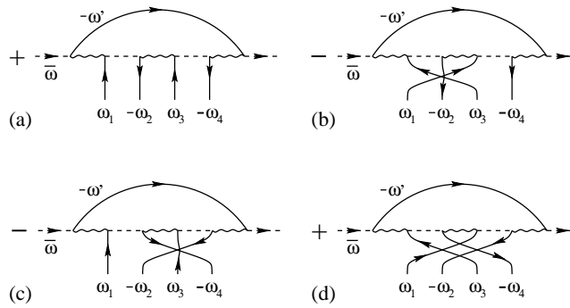
Fig. 9. Set of contributions to skeleton diagrams not contained in CTMA which cancel in the infrared limit to leading and subleading order in the external frequency, \omega \rightarrow 0 .
