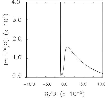
Fig. 4. Imaginary part of the conduction electron-pseudofermion T -matrix T^{(cf)} as a function of the COM frequency \Omega for the single-channel case M = 1 , N = 2 , evaluated by inserting NCA solutions for the intermediate state propagators ( E_d = -0.67D , \Gamma = 0.15D , T = 4 \cdot 10^{-3}T_K ). The contribution from the pole positioned at a negative frequency \Omega = \Omega_{cf} \simeq -T_K (compare text) is clearly seen.
