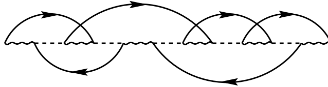
Fig. 8. Typical pseudofermion self-energy skeleton diagram of loop order L = 6 , containing L_{sp} = 1 spin (or fermion) loop and L_{ch} = 1 channel loop.
