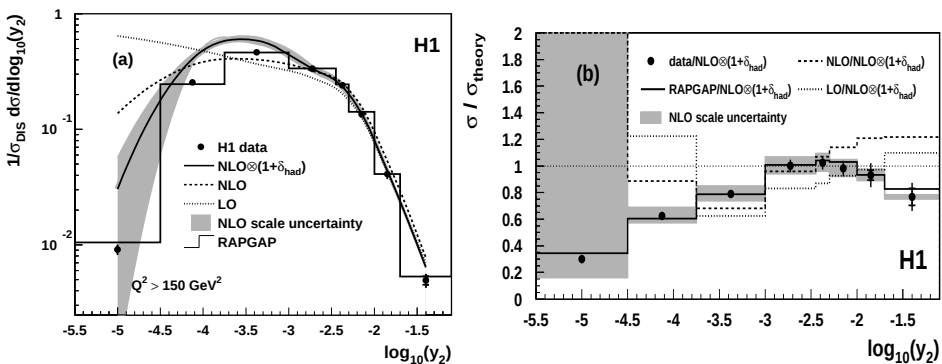
Fig. 1. (a) The normalized dijet cross section. Here and in the following figure the statistical errors are given by the inner error bars and the outer error bars correspond to the quadratic sum of the statistical and systematic errors. Also shown are perturbative QCD predictions in LO, in NLO with and without hadronization corrections, and the predictions of the QCD model RAPGAP. The shaded band shows the renormalization scale uncertainty of the NLO calculation. (b) The ratios of the data and various predictions. The vertical error bars correspond to the errors of the data only.
