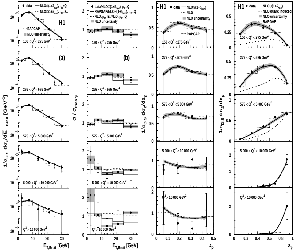
Fig. 2. The normalized dijet cross sections. The predictions of NLO QCD and RAPGAP are shown. The shaded band corresponds to the quadratic sum of the hadronization and renormalization scale uncertainties. (a) Besides the NLO QCD predictions with the scale \mu_R = Q , calculations with \mu_R = \bar{E}_{T,Breit} are also shown. (b) The ratios of the data and various predictions.
