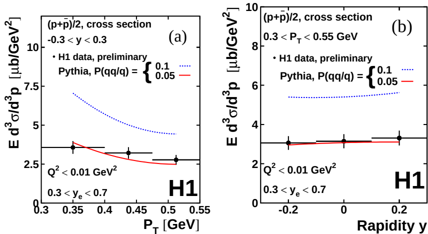
Fig. 2. The measured photoproduction cross-section E \frac{d^3\sigma}{d^3p} as a function of (a) transverse momentum p_T and (b) rapidity y , in the region of 0.3 < p_T < 0.55 GeV and -0.3 < y < 0.3 . The cross-section represents half of the sum of protons and anti-protons inclusively produced. The prediction of the PYTHIA model is shown with two different values of the diquark suppression factor, 0.1 (upper curve) and 0.05 (lower curve).
