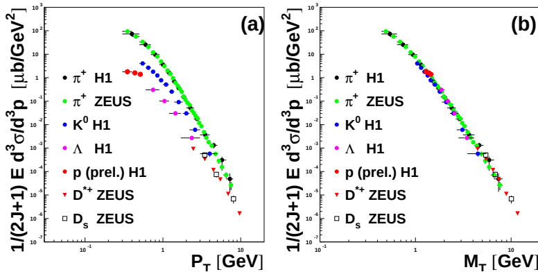
Fig. 3. Photoproduction cross section E \frac{d^3\sigma}{d^3p} for different hadrons as a function of (a) transverse momentum p_T and (b) transverse mass M_T (= m + p_T) , in the central rapidity region as measured in the laboratory frame of reference. The cross-sections are given for one isospin and corrected for the spin.
