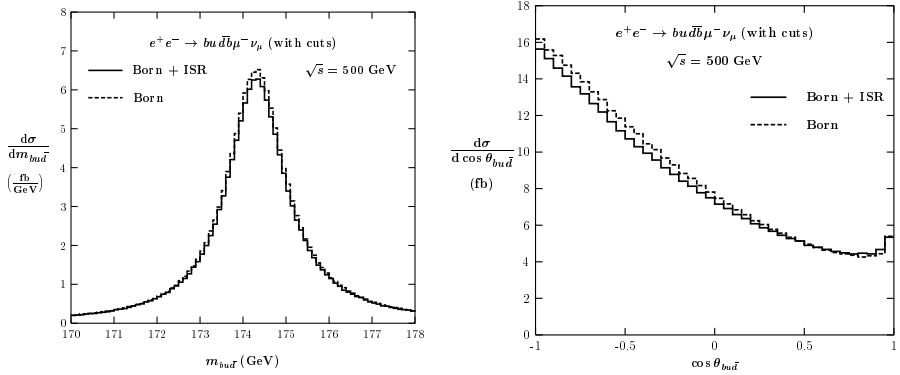
Fig. 1. Invariant mass (left) and angular (right) distributions of a \bar{b}d\bar{u} -quark triple at \sqrt{s} = 500 GeV with cuts.
