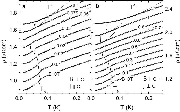
Fig. 4. Low-temperature electrical resistivity of YbRh 2 Si 2 at varying magnetic fields applied perpendicular (a) and along the c -axis (b). For clarity the different curves in B > 0 were shifted subsequently by 0.1 \mu\Omega\text{cm} . Up- and down-raising arrows indicate T_N and upper limit of T^2 behavior, respectively. Dotted and solid lines represent \Delta\rho \sim T^\varepsilon with \varepsilon = 1 and \varepsilon = 2 , respectively.
