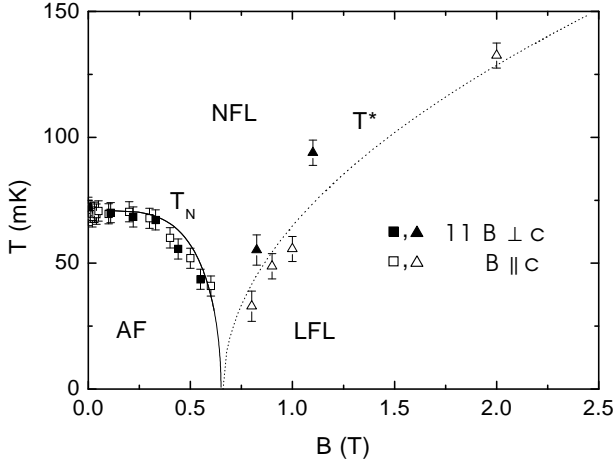
Fig. 5. T - B phase diagram for YbRh 2 Si 2 with T_N as derived from d\rho/dT vs T and T^* , the upper limit of the \Delta\rho = AT^2 behavior, as a function of magnetic field, applied both along and perpendicular to the c -axis. For the latter ones the B -values have been multiplied by a factor 11. Lines separating the antiferromagnetic (AF), non-Fermi liquid (NFL) and Landau Fermi liquid (LFL) phase are guides to the eye.
