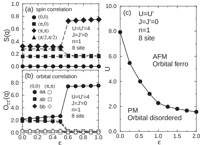
Fig. 1. (a) Spin and (b) orbital correlations as a function of \varepsilon . (c) Ground-state phase diagram for n=1 with U=U' and J=J'=0 .
