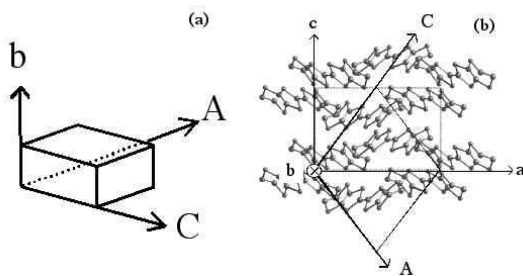
Fig. 1. (a) Crystal orientation of the sample measured in this work and (b) crystal structure of \kappa\text{-(ET)}_2\text{Cu[N(CN)}_2\text{]Br} .
