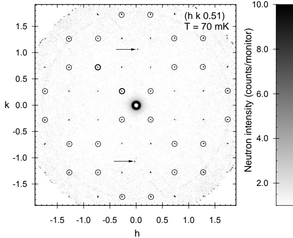
Fig. 1. Intensity map of the reciprocal (h k 0.51) plane in \text{CeCu}_2(\text{Si}_{0.5}\text{Ge}_{0.5})_2 at T = 70 mK. The peaks surrounded by circles are magnetic satellites of (h k 0) nuclear peaks, while the other magnetic peaks originate from (h k 1) nuclear peaks. Two spurious nuclear peaks not connected to the magnetic structure are marked by arrows. The temperature dependence of the magnetic order was measured on the two magnetic peaks specially indicated by thick circles and they are referred to as (000)^+ and (110)^+ .
