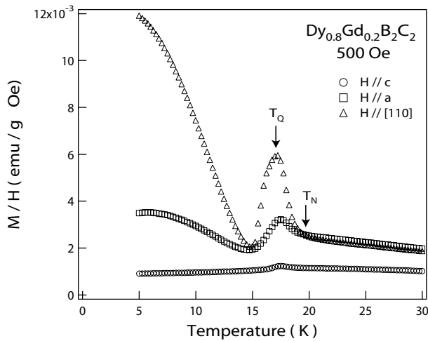
Fig. 2. Temperature dependence of the magnetizations of \text{Dy}_{0.8}\text{Gd}_{0.2}\text{B}_2\text{C}_2 .
