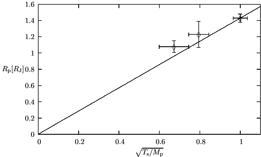
Fig. 1. The measured effective size, R_p , of the transiting planets HD209458b, OGLE-TR-56b and OGLE-TR-113b versus \sqrt{T_s/M_p} (in units where \sqrt{T_s/M_p} = 1 for HD209458b). The straightline is the prediction, Eq. (1), which assumes that the planets are composed predominately of mirror matter.
