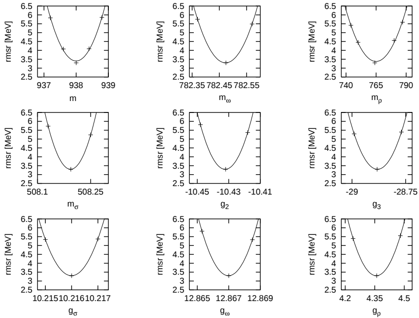
Fig. 1. Rms deviation of the macroscopic NL4 RMFT energies from those of the LSD model as function of each of the RMFT parameters.
