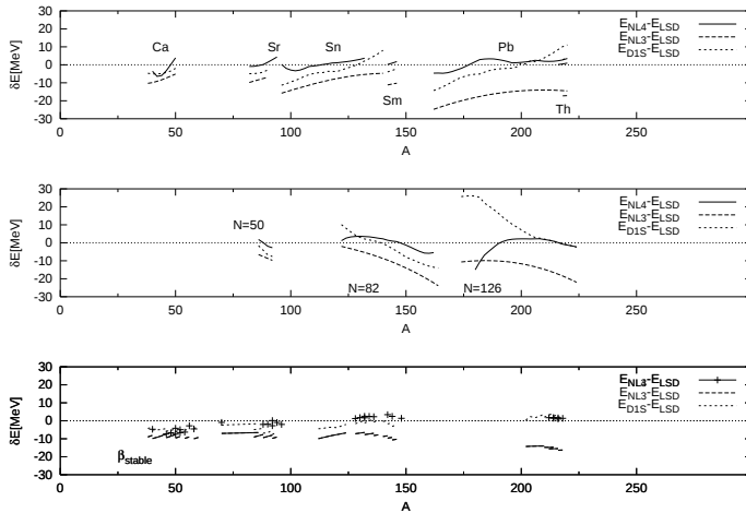
Fig. 2. The deviations of the macroscopic energies obtained in the LSD model, and, on the other hand, in the RMFT with the NL3, NL4 parameter sets or with the Gogny D1S effective interaction for 142 spherical even-even isotopes (top), isotones (middle) and \beta stable nuclei (bottom) as function of mass number A .
