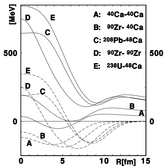
Fig. 3 (corrected). Potentials \mathcal{V} (broken curves) and \mathcal{V}_{\text{tot}} (solid curves) between the indicated pairs of nuclei at K_r = 1.5 \text{ fm}^{-1} .
