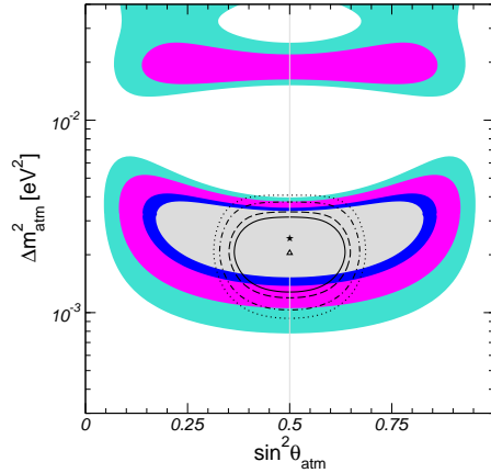
Fig. 1. Allowed regions for \sin^2 \theta_{23} and \Delta m_{31}^2 at 90%, 95%, 99%, and 3\sigma C.L. for atmospheric neutrino data (contour lines) and the K2K long-baseline experiment (colored regions).
