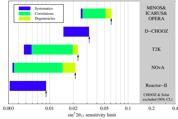
Fig. 5. Sensitivity to \sin^2 2\theta_{13} at 90% C.L. The left edges of the bars are obtained for the statistics limits only, whereas the right edges are obtained after successively switching on systematics, correlations, and degeneracies, i.e. , they correspond to the final sensitivity. The gray shaded region is excluded at 90% C.L. by present data. For the true values of the oscillation parameters, we use \Delta m_{31}^2 = +2.0 \times 10^{-3} \text{ eV}^2 , \sin^2 2\theta_{23} = 1 , \Delta m_{21}^2 = 7.0 \times 10^{-5} \text{ eV}^2 , \sin^2 2\theta_{12} = 0.8 .
