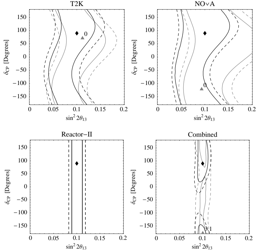
Fig. 6. The 90% C.L. (solid) and 3\sigma (dashed) allowed regions (2 d.o.f.) in the \sin^2 2\theta_{13} - \delta_{\text{CP}} plane for the true values \sin^2 2\theta_{13} = 0.1 and \delta_{\text{CP}} = 90^\circ . The black curves refer to the allowed regions for the normal mass hierarchy (assumed to be the true hierarchy), whereas the gray curves refer to the \text{sgn}(\Delta m_{31}^2) -degenerate solution (inverted hierarchy), where the projections of the minima onto the \sin^2 2\theta_{13} - \delta_{\text{CP}} plane are shown as diamonds (normal hierarchy) and triangles (inverted hierarchy). For the latter, the \Delta\chi^2 -value with respect to the best-fit point is also given.
