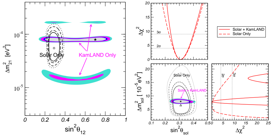
Fig. 2. Left: Allowed regions for \sin^2 \theta_{12} and \Delta m_{21}^2 at 90%, 95%, 99%, and 3\sigma C.L. for solar neutrino data (contour lines) and the KamLAND reactor experiment (colored regions). Right: Combined solar+KamLAND analysis. Also shown is the allowed region from solar data only (contour lines).
