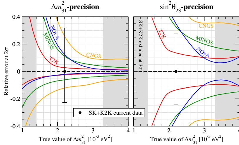
Fig. 4. Prospective relative errors at 2\sigma on |\Delta m_{31}^2| (left) and \sin^2 \theta_{23} (right) as a function of the true value of \Delta m_{31}^2 and for the true value \sin^2 \theta_{23} = 0.5 . The dots with the error bars indicate the present accuracy at 2\sigma from atmospheric and K2K data. The gray shaded region is excluded at 3\sigma by present data.
