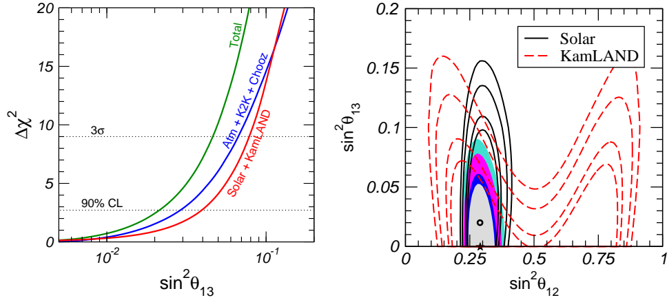
Fig. 3. Left: \Delta\chi^2 as a function of \sin^2 \theta_{13} for solar+KamLAND, CHOOZ+atmospheric+K2K, and global data. Right: Allowed regions for \sin^2 \theta_{12} and \sin^2 \theta_{13} at 90%, 95%, 99%, and 3\sigma C.L. for solar neutrino data (solid contour lines), KamLAND (dashed contour lines), and solar+KamLAND data (colored regions).
