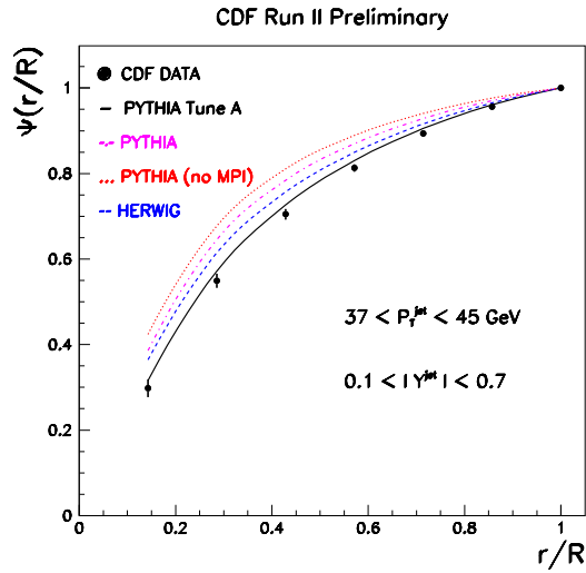
Fig. 7. The measured integral jet shape, \Psi(r/R) , in inclusive jet production for jets with 0.1 < |\gamma^{\text{jet}}| < 0.7 and 37 \text{ GeV}/c < P_T^{\text{jet}} < 45 \text{ GeV}/c .
