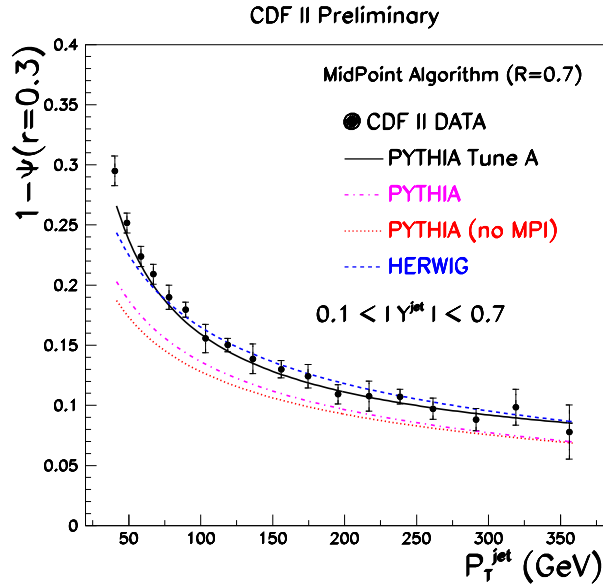
Fig. 9. The measured integral jet shape, 1 - \Psi(0.3/R) , as function of P_T^{\text{jet}} in comparison to various Monte Carlo predictions.
