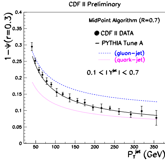
Fig. 10. The measured integral jet shape, 1 - \Psi(0.3/R) , as function of P_T^{\text{jet}} in comparison to Pythia-Tune A predictions for gluon and quark jets.
