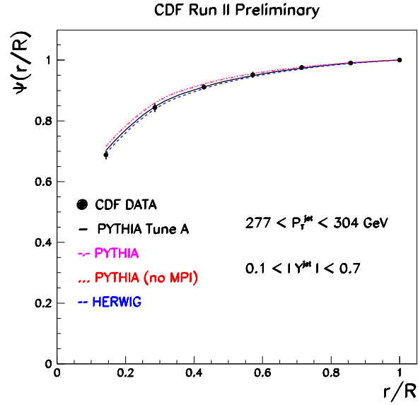
Fig. 8. The measured integral jet shape, \Psi(r/R) , in inclusive jet production for jets with 0.1 < |\gamma^{\text{jet}}| < 0.7 and 277 \text{ GeV}/c < P_T^{\text{jet}} < 304 \text{ GeV}/c .
