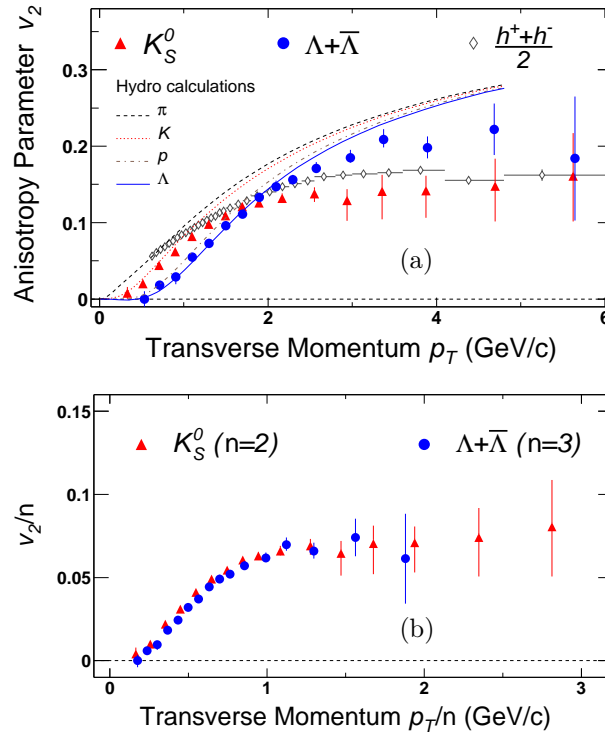
Fig. 4. Transverse momentum dependence of elliptic flow v_2 measured by STAR [55] (a) before and (b) after rescaling by the number of valence quarks n .
