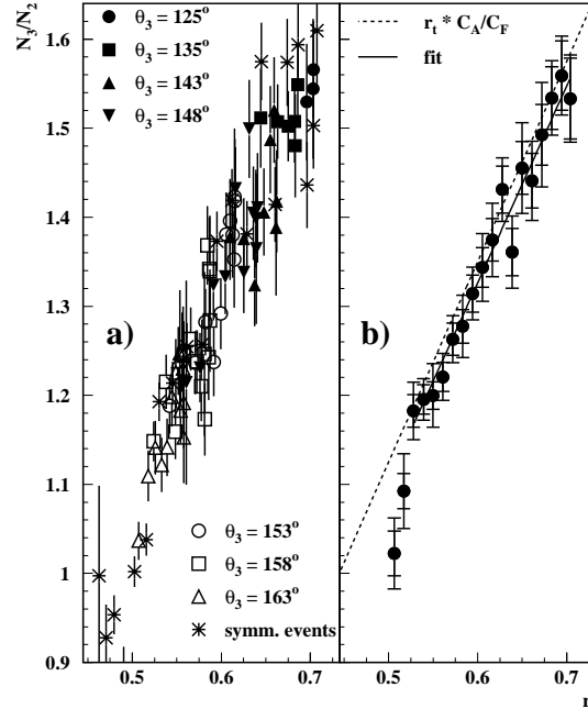
Fig. 2. Multiplicity ratio N_3/N_2 in cones of 30^\circ opening angle as function of r_t in Eq. (2): (a) for different inter-jet angles \theta_3 ; (b) averaged over \theta_3 , the dashed line is the expectation Eq. (2) with slope C_A/C_F , the full line is a fit (DELPHI [27]).
