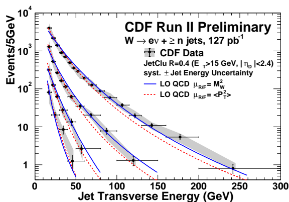
Fig. 1. Distribution of the jet E_T for the jet of lowest energy in the W + \geq n jet sample, for n = 1 (top) to n = 4 (down), in comparison with LO QCD calculations.
