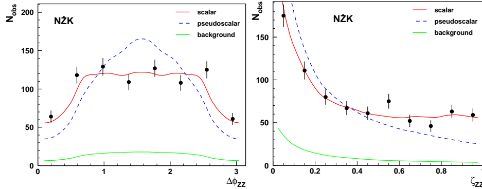
Fig. 5. Measurement of the angle \Delta\phi_{ZZ} between two Z -decay planes (left plot) and of the variable \zeta_{ZZ} calculated from the polar angles of the Z \rightarrow l^+l^- and Z \rightarrow jj decays (right plot) for ZZ \rightarrow l^+l^-jj events. Points with error bars indicate the statistical precision of the measurement after one year of Photon Collider running at nominal luminosity. The solid and dashed lines correspond to predictions of the model with pure scalar ( \Phi_{\text{CP}} = 0 ) and pseudoscalar ( \Phi_{\text{CP}} = \pi/2 ) Higgs-boson couplings, respectively. Grey line represents the SM background of non-resonant ZZ production. Signal and background calculations are performed for primary electron-beam energy of 152.5 GeV and the Higgs-boson mass of 200 GeV.
