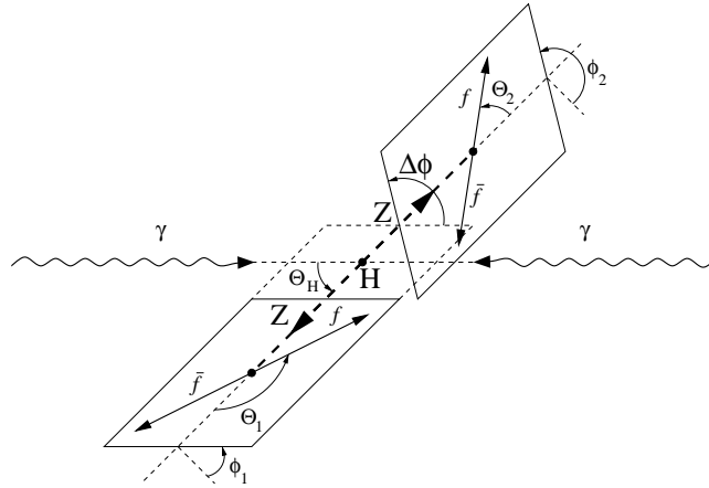
Fig. 1. The definition of the polar angles \Theta_H , \Theta_1 and \Theta_2 , and the azimuthal angles \phi_1 and \phi_2 for the process \gamma\gamma \rightarrow h \rightarrow ZZ \rightarrow 4f . \Delta\phi is the angle between two Z decay planes, \Delta\phi = \phi_2 - \phi_1 . All polar angles are calculated in the rest frame of the decaying particle.
