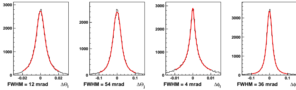
Fig. 3. Resolution in the reconstructed Z -decay angles \Theta and \phi , for the leptonic ( \Theta_l , \phi_l ) and hadronic ( \Theta_j , \phi_j ) final states. Events were simulated with the PYTHIA and SIMDET programs, for a primary electron-beam energy of 209 \text{ GeV} and Standard Model Higgs-boson mass of 300 \text{ GeV} .
