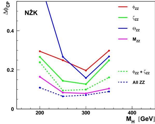
Fig. 7. Statistical error in the determination of \Phi_{CP} , expected after one year of Photon Collider running, as a function of the Higgs-boson mass M_H . Fits were performed to the shape of the three individual angular distributions measured for ZZ events, as indicated in the plot, and to the reconstructed invariant mass distribution. Results of the simultaneous fits to three angular distributions and to all distributions are also shown. All other parameters, except for the overall normalisation, are fixed to the Standard Model values. Errors were calculated assuming \Phi_{CP} \approx 0 .
