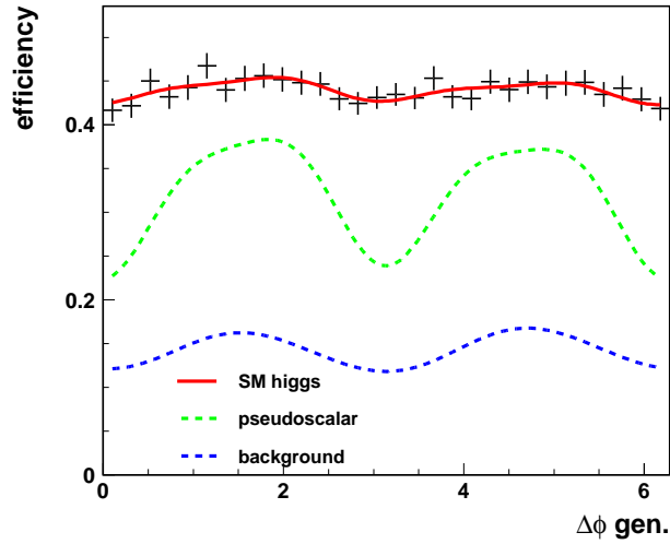
Fig. 4. Selection efficiency as a function of the angle \Delta\phi between two Z decay planes, for ZZ \rightarrow l^+l^-jj events coming from the scalar Higgs decays, pseudoscalar Higgs decays and non-resonant background. Events were simulated with the PYTHIA and SIMDET programs, for a primary electron-beam energy of 209 GeV and Higgs-boson mass of 300 GeV. Only events with the reconstructed Higgs mass between 286 and 312 GeV are accepted.
