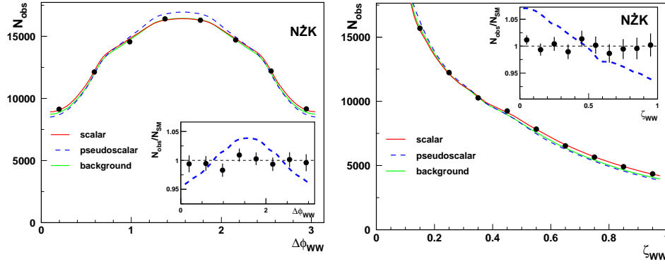
Fig. 6. Measurement of the angle \Delta\phi_{WW} between two W -decay planes (left plot) and of the variable \zeta_{WW} calculated from the polar angles of two W \rightarrow jj decays (right plot) for WW \rightarrow 4j events. Points with error bars indicate the statistical precision of the measurement after one year of Photon Collider running at nominal luminosity. The solid and dashed lines correspond to predictions of the model with pure scalar ( \Phi_{\text{CP}} = 0 ) and pseudoscalar ( \Phi_{\text{CP}} = \pi/2 ) Higgs-boson couplings, respectively. Grey line represents the SM background of non-resonant W^+W^- production. Signal and background calculations are performed for primary electron-beam energy of 152.5 GeV and the Higgs-boson mass of 200 GeV. The insets show the relative deviations from the Standard Model predictions ( \Phi_{\text{CP}} = 0 ) for pseudoscalar Higgs-boson couplings.
