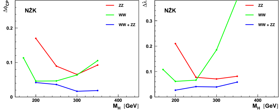
Fig. 8. Statistical error in the determination of \Phi_{\text{CP}} (left plot) and \lambda (right plot), expected after one year of Photon Collider running, as a function of the Higgs-boson mass M_H . Combined fits were performed to the considered angular distributions and invariant mass distributions for ZZ events and W^+W^- events. Results were obtained assuming small deviations from Standard Model predictions, i.e. \lambda \approx 1 and \Phi_{\text{CP}} \approx 0 . Two photon width of the Higgs-boson, \Gamma_{\gamma\gamma} , the phase \phi_{\gamma\gamma} and normalisations of both samples are allowed to vary in the fit.
