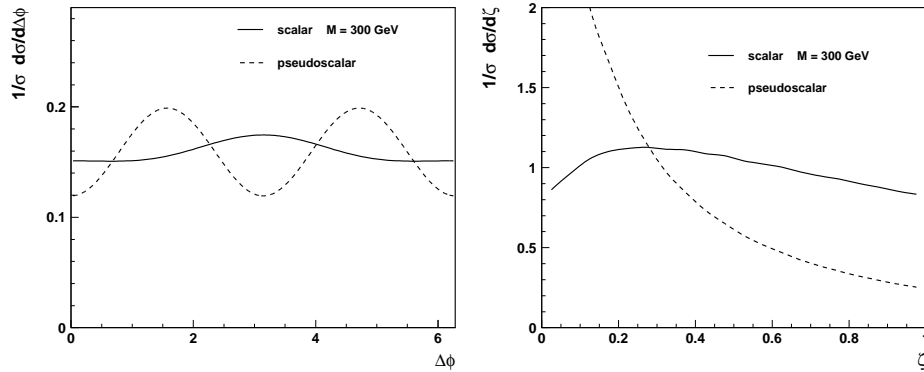
Fig. 2. Normalised angular distributions in \Delta\phi (left plot) and \zeta (right plot), expected for scalar and pseudoscalar Higgs decays H, A \rightarrow ZZ \rightarrow l^+l^-jj , for the Higgs mass of 300 GeV.
