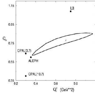
Fig. 2. Figure from Ref. [7] where it is presented the \Delta\chi^2 = 1 contour in the (Q_0^2, C_{np}) plane as well as the individual best fits for each LEP experiment. The point for DELPHI(12.7) is outside the figure, while for DEPHI (3.7) no minimum is found for Q_0^2 < 1.9 \text{ GeV}^2 .
