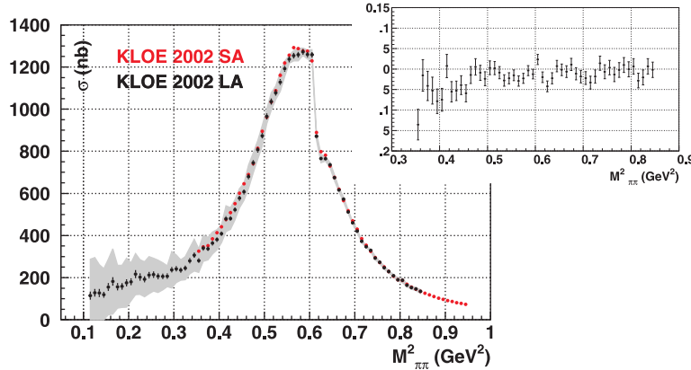
Fig. 3. Spectra and relative difference (inlay) of the small angle (SA) and large angle (LA) analyses for 2002 data; the grey error band indicates the model uncertainty in subtracting the irreducible \phi \rightarrow f_0(980)\gamma background in the large angle analysis.
