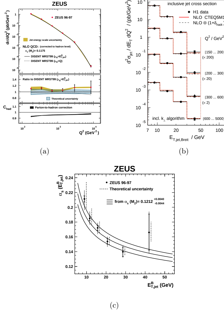
Fig. 1. (a) Inclusive-jet cross section in NC DIS as a function of Q^2 [1]; (b) inclusive-jet cross section in NC DIS as a function of E_{T,B}^{jet} in different regions of Q^2 [2]; (c) energy-scale dependence of \alpha_s [1].
