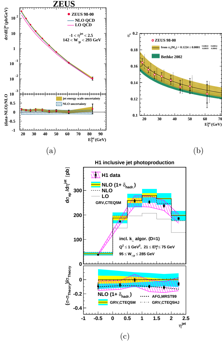
Fig. 6. (a) Inclusive-jet cross section as a function of E_T^{\text{jet}} [8]; (b) \alpha_s as a function of E_T^{\text{jet}} [8]; (c) inclusive-jet cross sections as a function of \eta^{\text{jet}} [9].
