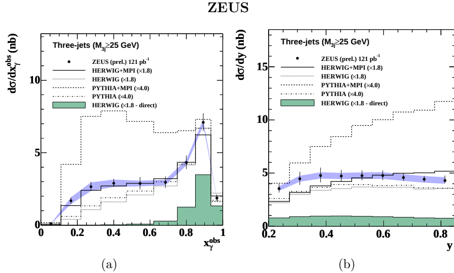
Fig. 7. Three-jet cross sections in PHP for M^{3j} > 25 GeV as functions of (a) x_\gamma^{\text{obs}} and (b) y [14]. For comparison, the predictions of PYTHIA and HERWIG with and without MPIs are included.
