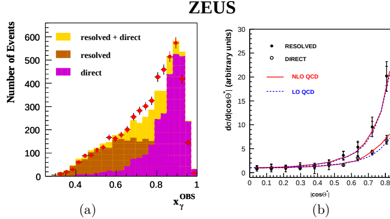
Fig. 5. (a) x_\gamma^{\text{obs}} distribution for data and resolved, direct and resolved+direct MC events [7]; (b) Dijet cross section as a function of |\cos \theta^*| in PHP for x_\gamma^{\text{obs}} \leq 0.75 [7].
