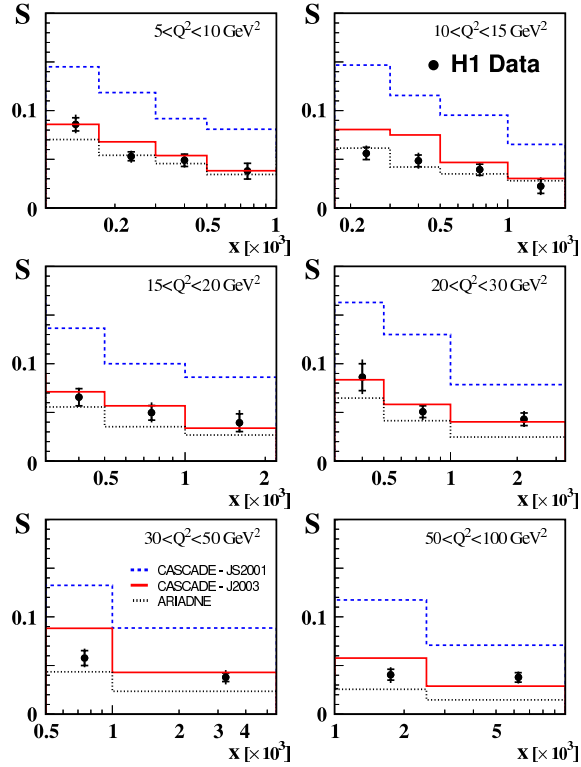
Fig. 4. Azimuthal correlation as a function of x for different Q^2 regions [6] compared to the CDM and CASCADE MC predictions.
