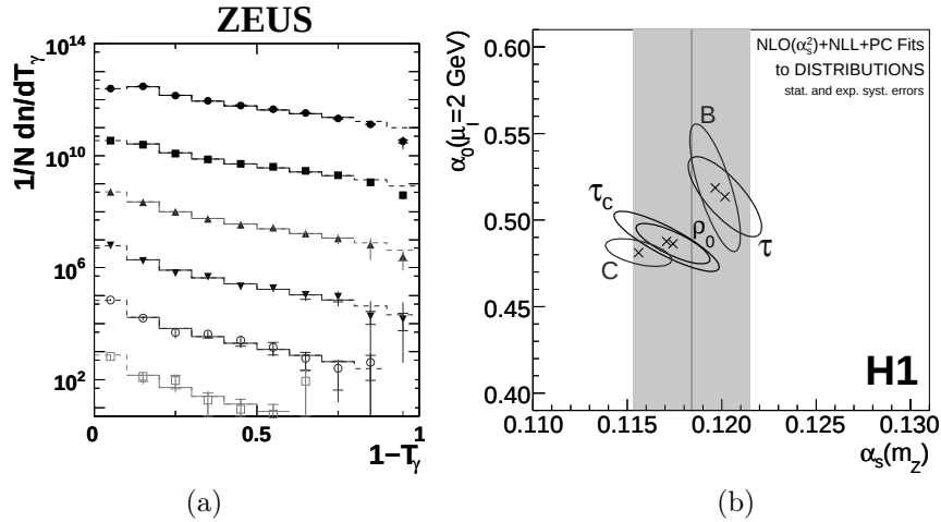
Fig. 2. (a) Thrust distribution in different Q^2 regions [3]; (b) \bar{\alpha}_0 and \alpha_s(M_Z) values extracted from event-shape distributions [4].
