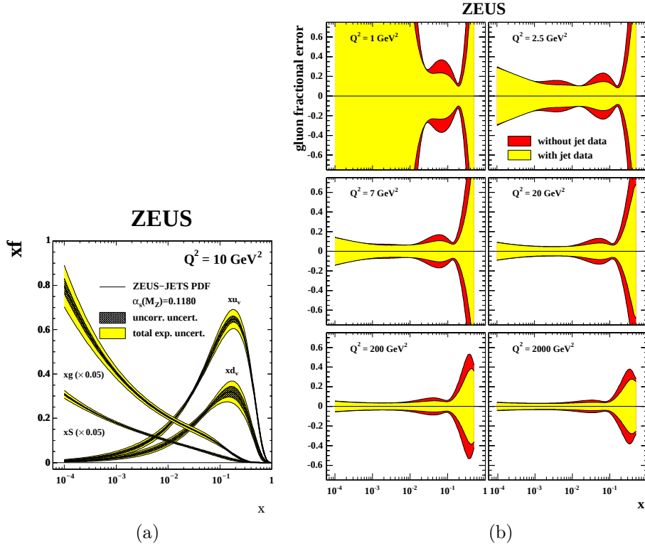
Fig. 9. (a) Valence, sea and gluon distributions from the ZEUS-jets proton PDF parametrisations [13]; (b) uncertainties of the ZEUS-jets proton PDF parametrisations [13].
