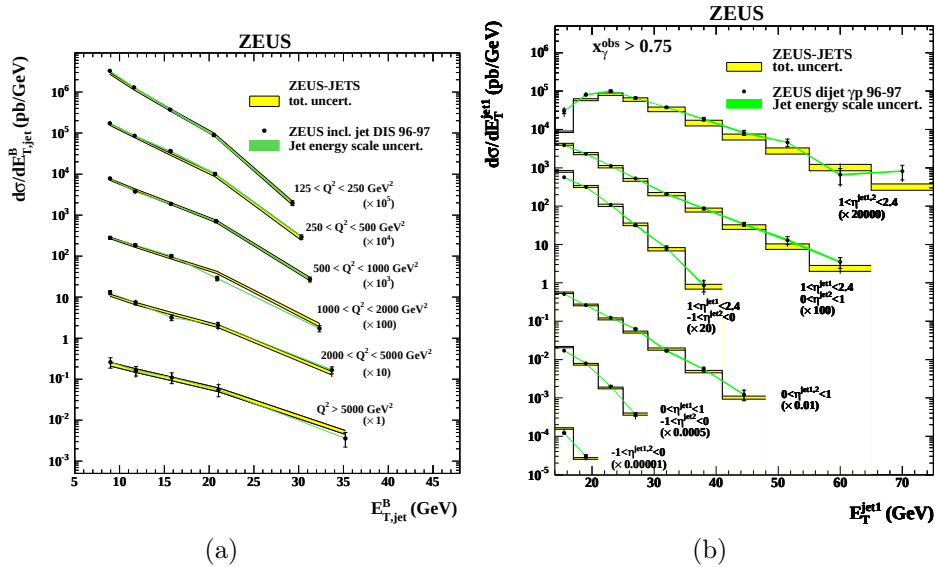
Fig. 8. (a) Inclusive-jet cross section in NC DIS as a function of E_{T,B}^{\text{jet}} in different regions of Q^2 [1]; (b) Dijet cross section in PHP as a function of E_T^{\text{jet}} in different regions of \eta^{\text{jet}} for x_{\gamma}^{\text{obs}} > 0.75 [7]. Both measurements are compared to NLO calculations based on ZEUS-jets proton PDFs [13].
