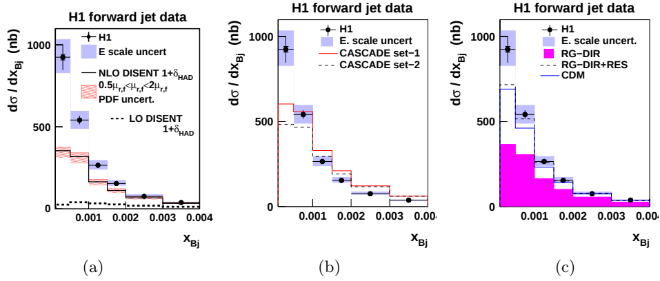
Fig. 3. Forward-jet cross section as a function of Bjorken x [5] compared to (a) LO and NLO calculations; (b) CASCADE MC predictions; and (c) CDM and RAPGAP MC predictions.
