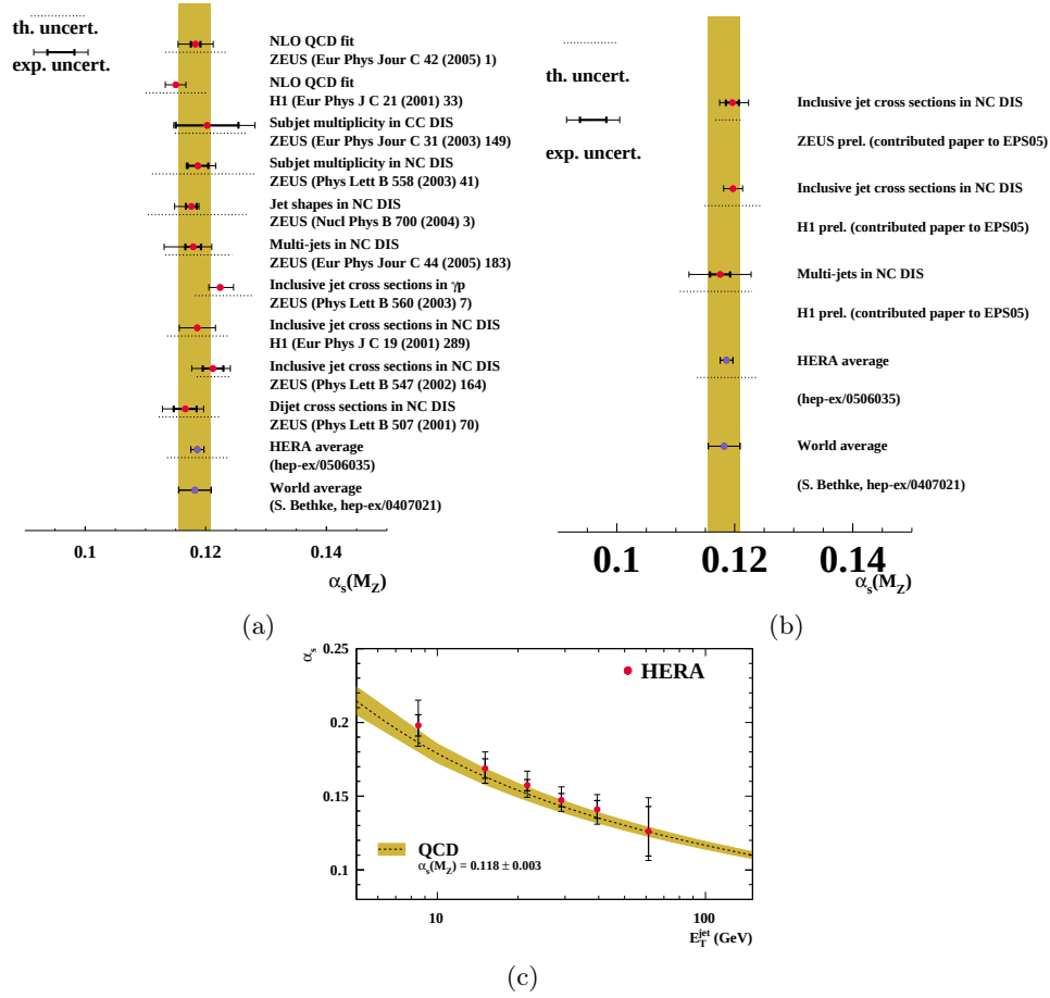
Fig. 10. (a,b) Summary of \alpha_s(M_Z) measurements at HERA compared with the world and HERA averages [11]; (c) combined measurements of \alpha_s(E_T^{\text{jet}}) from HERA [11].
