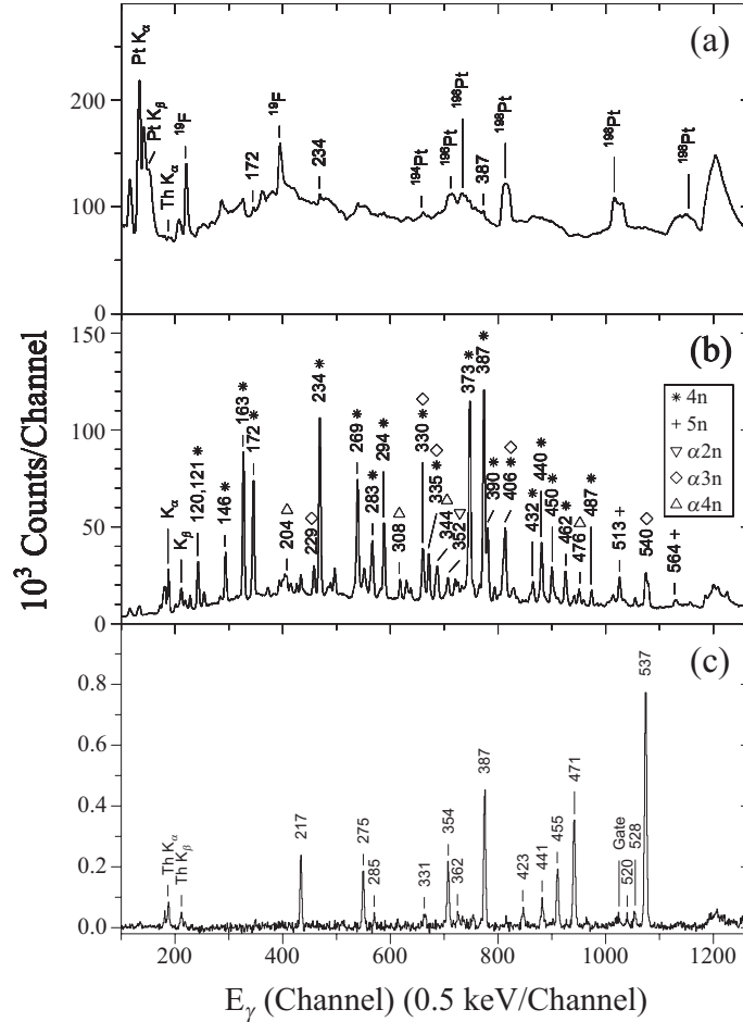
Fig.1. Sample \gamma -ray energy spectra for the 128-MeV ^{26}\text{Mg} + ^{198}\text{Pt} reaction. (a) The “raw” spectrum. A fraction of the data is shown. (b) The projection of a residue-gated \gamma - \gamma coincidence matrix. Transitions are labeled by their energies in keV and symbols for the evaporation channels. The composite K X-ray peaks are also visible. (c) A residue- and \gamma -ray gated coincidence spectrum.
