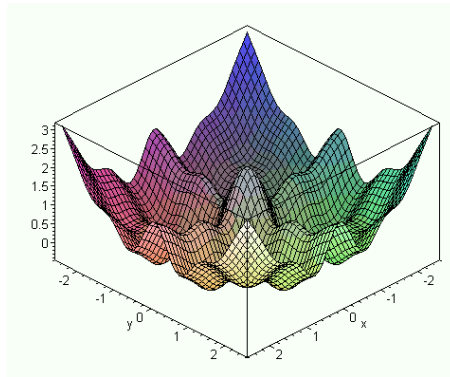
Fig. 1. Fahy–Hamann potential.
