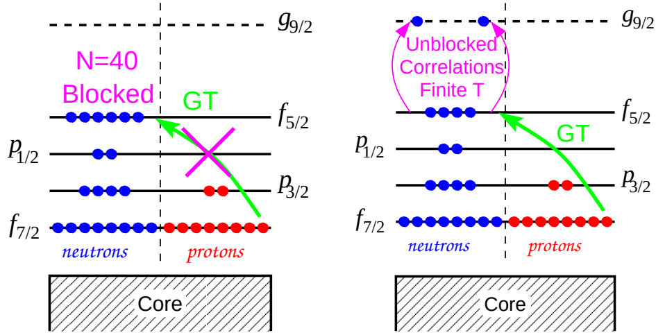
Fig. 3. In the independent particle model GT transitions are blocked at neutron number N = 40 .
