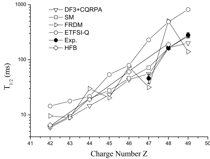
Fig. 10. Comparison of various theoretical half-life predictions with data for the N = 82 r-process waiting points (from [56]).
