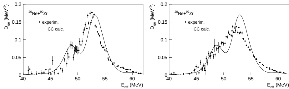
Fig. 1. Barrier height distributions for ^{20}\text{Ne} + ^{90}\text{Zr} (left panel) and ^{20}\text{Ne} + ^{92}\text{Zr} (right panel) compared with the results of coupled channels calculations (Ref. [4]).
