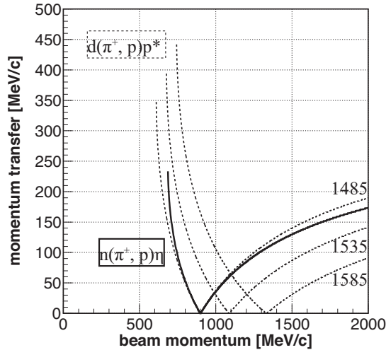
Fig. 4. Momentum transfer for the n(\pi^+, p)\eta reaction (solid line) and the d(\pi^+, p)p^* reaction (dashed lines) for three different p^* masses (1485, 1535 and 1585 MeV/ c^2 ).
