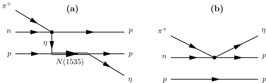
Fig. 3. Diagrams for the \pi^+ d \rightarrow pp\eta reaction, (a) double-scattering reaction, (b) quasi-free reaction.
