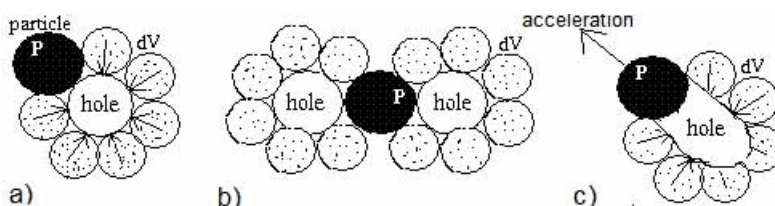
Fig. 1. (a) The interaction of particle P with a hole; (b) the interaction of particle P with two holes; (c) Particle P moves with acceleration and “expands” a hole.
