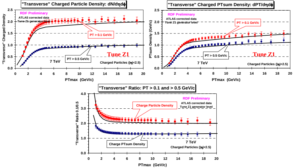
Fig. 18. ATLAS data at 7 TeV [16] on the transverse charged particle density (top left) and the transverse charged PTsum density (top right) as defined by the leading charged particle, PTmax, as a function of PTmax for charged particles with p_T > 0.5 GeV/c and |\eta| < 2.5 and for charged particles with p_T > 0.1 GeV/c and |\eta| < 2.5 . The data are corrected to the particle level and compared with PYTHIA Tune Z1 at the generator level. (bottom) Ratio of the ATLAS data with p_T > 0.1 GeV/c and p_T > 0.5 GeV/c (100 MeV/c cut divided by 500 MeV/c cut) for the transverse charged particle density and the charged PTsum density as defined by the leading charged particle, PTmax, as a function of PTmax compared with PYTHIA Tune Z1.
