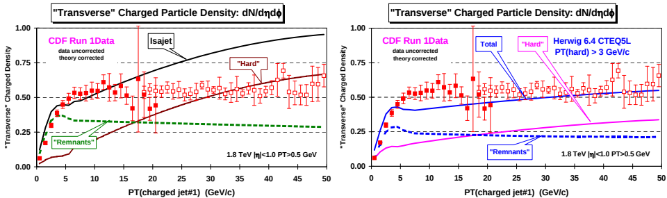
Fig. 2. CDF Run 1 data from Ref. [1] at 1.8 TeV on the density of charged particles ( p_T > 0.5 GeV/c, |\eta| < 1 ) in the “transverse” region as defined by the leading charged particle jet, chgjet#1, as a function of P_T(\text{chgjet}\#1) . The data are compared with ISAJET 7.32 without MPI (left) and HERWIG 6.4 without MPI (right) using the ISAJET and HERWIG default parameters with p_T(\text{hard}) > 3 GeV/c. The Monte Carlo predictions are divided into two categories: charged particles that arise from the break-up of the beam and target (beam-beam remnants); and charged particles that arise from the outgoing jets plus initial and final-state radiation (hard scattering component).
