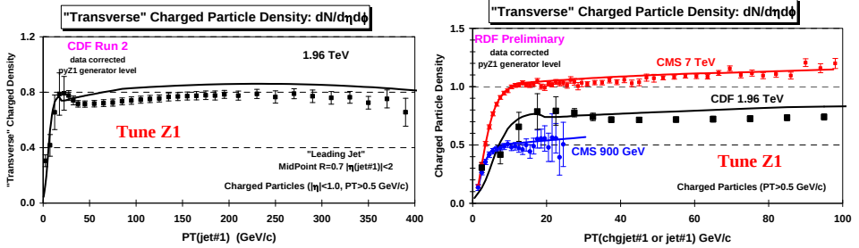
Fig. 19. (left) CDF data at 1.96 TeV from Ref. [13] on the charged particle density ( p_T > 0.5 GeV/c, |\eta| < 1 ) in the “transverse” region as defined by the leading calorimeter jet, jet#1, as a function of P_T(\text{jet}\#1) compared with PYTHIA Tune Z1. Also compares the CDF data at 1.96 TeV with the CMS data [14] at 900 GeV and 7 TeV (right) on the “transverse” charged particle density ( p_T > 0.5 GeV/c, |\eta| < 2 ) in the “transverse” region as defined by the leading charged particle jet, chgjet#1, as a function of P_T(\text{chgjet}\#1) . The data are corrected to the particle level and compared with PYTHIA Tune Z1 at the generator level.
