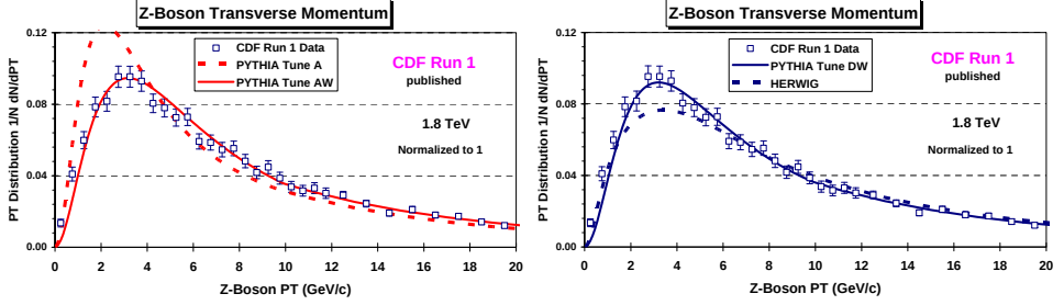
Fig. 5. The CDF Run 1 data from Ref. [8] on the Z -boson p_T distribution ( \langle p_T(Z) \rangle \approx 11.5 GeV/c) compared with (left) PYTHIA Tune A ( \langle p_T(Z) \rangle = 9.7 GeV/c) and PYTHIA Tune AW ( \langle p_T(Z) \rangle = 11.7 GeV/c) and compared with (right) PYTHIA Tune DW and HERWIG 6.4 (without MPI).
