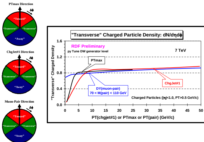
Fig. 8. Shows the charged particle density in the “transverse” region for charged particles ( p_T > 0.5 GeV/c, |\eta| < 1 ) at 7 TeV as defined by PT_{max} , P_T(chgjet\#1) , and P_T(muon-pair) predicted from PYTHIA Tune DW at the particle level. For muon-pair production the two muons are excluded from the charged particle density. Charged particle jets are constructed using the Anti-KT algorithm with d = 0.5 .
