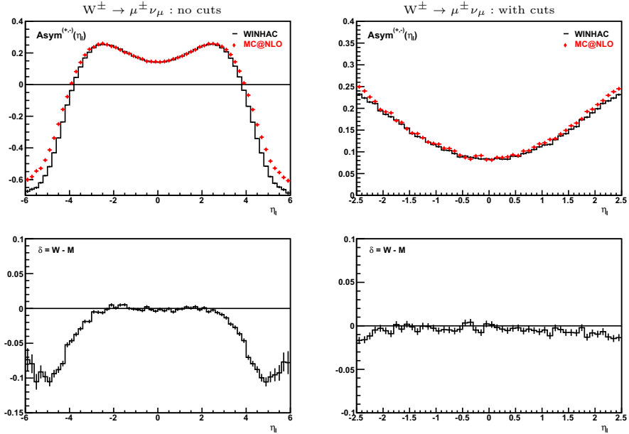
Fig. 3. The \eta_l charge asymmetries from WINHAC and MC@NLO without cuts (left plots) and with the typical ATLAS and CMS cuts (right plots); lower plots show the differences between the programs.
