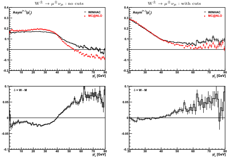
Fig. 8. The p_T^l charge asymmetries from WINHAC without rotations of leptons momenta in the W -rest frame and MC@NLO, without cuts (left plots) and with the typical ATLAS and CMS cuts (right plots); lower plots show the differences between the programs.
