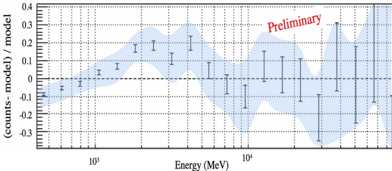
Fig. 4. Residuals ((\text{exp. data} - \text{model})/\text{model}) of the above likelihood analysis. The shaded (blue) area shows the systematic errors on the effective area.
