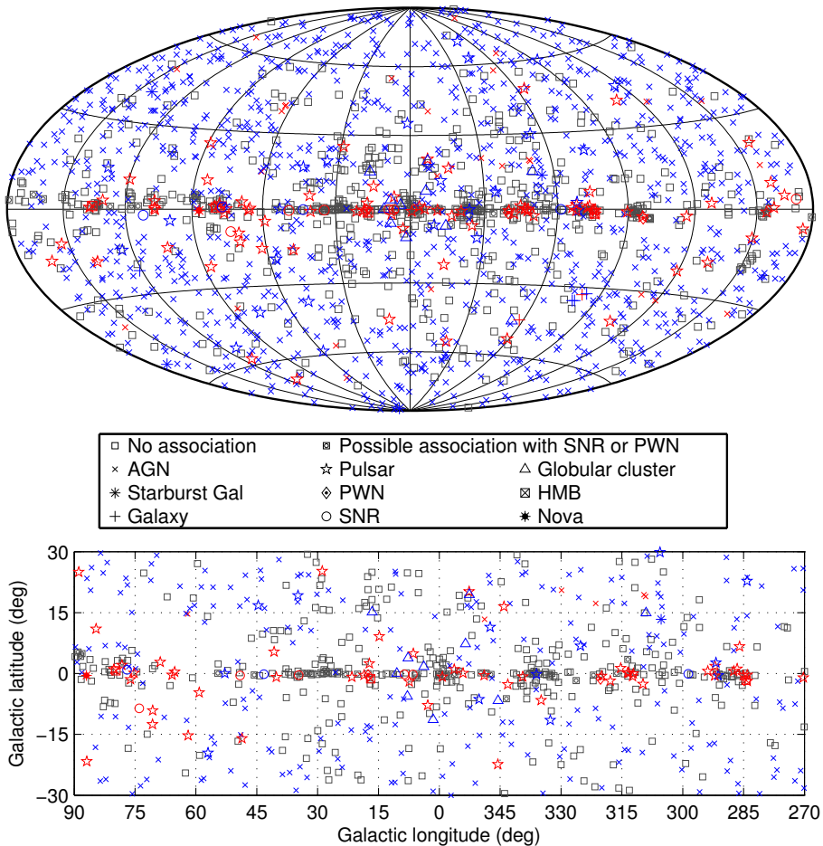
Fig. 2. Full sky map (top) and blow-up of the inner Galactic region (bottom) showing sources by source class. Identified sources are shown with a grey (red) symbol, associated sources in black (blue).
