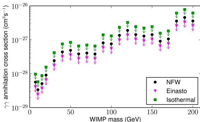
Fig. 8. Dark Matter annihilation 95% C.L. cross section upper limits into \gamma\gamma for the NFW, Einasto, and isothermal profiles for the region |b| > 10^\circ plus a 20^\circ \times 20^\circ square at the GC.
