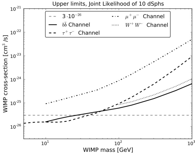
Fig. 5. Derived 95% C.L. upper limits on WIMP annihilation cross sections for different channels.
