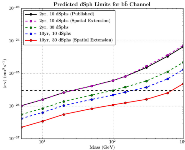
Fig. 7. Predicted 95% C.L. upper limits on WIMP annihilation cross sections in 10 years for b\bar{b} channel.
