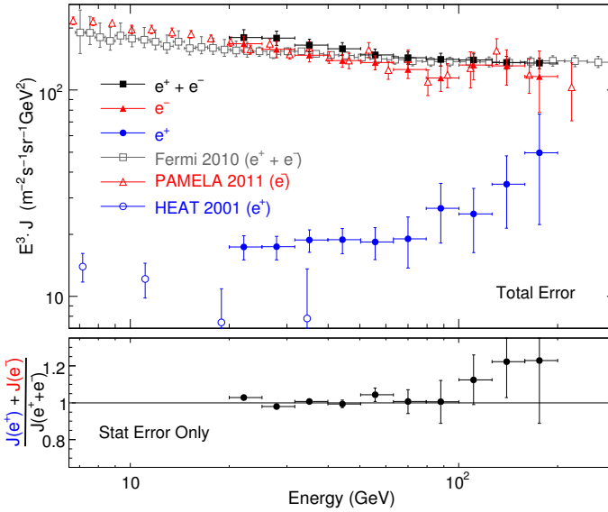
Fig. 9. Energy spectra for e^+ , e^- , and e^+ + e^- (control region). In the control region, where both species are allowed, this analysis reproduces the Fermi LAT results reported previously for the total electron plus positron spectrum [24, 25] (grey). Previous results from HEAT [27] and PAMELA [26] are shown for reference. The bottom panel shows that the ratio between the sum and the control flux is consistent with 1 as expected.
