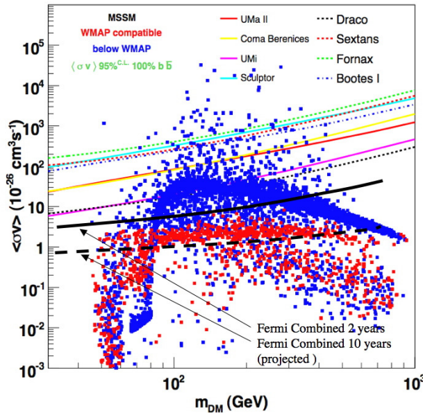
Fig. 6. MSSM models in the (m_{\text{wimp}}, \langle\sigma v\rangle) plane. The models are consistent with all accelerator constraints and light grey (red) points have a neutralino thermal relic abundance corresponding to the inferred cosmological Dark Matter density (dark grey (blue) points have a lower thermal relic density, and we assume that neutralinos still comprise all of the Dark Matter in virtue of additional non-thermal production processes.
