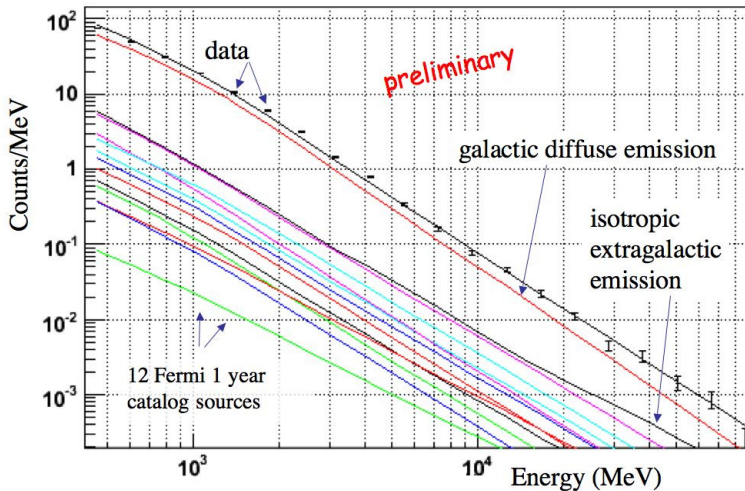
Fig. 3. Spectra from the likelihood analysis of the Fermi LAT data (number of counts versus reconstructed energy) in a 7^\circ \times 7^\circ region around the Galactic Center (number of counts versus reconstructed energy).
