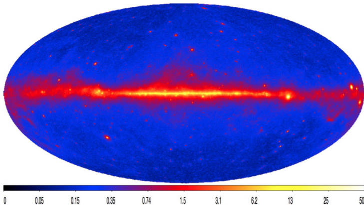
Fig. 1. Sky map of the energy flux derived from 24 months of observation. The image shows \gamma -ray energy flux for energies between 100 MeV and 10 GeV, in units of 10^{-7} \text{ erg cm}^{-2} \text{ s}^{-1} \text{ sr}^{-1} .
