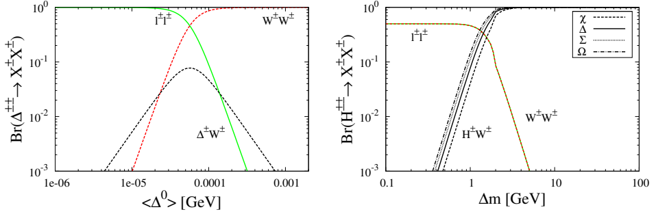
Fig. 2. Left: Scalar branching ratios for the triplet \Delta as a function of \langle\Delta^0\rangle for \sum_{i=1,2,3} m_{\nu_i}^2 = 0.1^2 \text{ eV}^2 and m_{\Delta^{\pm\pm}} = 500 \text{ GeV} , and \Delta m = 1 \text{ GeV} for the decay into \Delta^{\pm}W^{\pm*} \rightarrow \Delta^{\pm}e^{\pm}\nu_e, \dots . Right: Scalar branching ratios for different H multiplets as a function of \Delta m = m_{H^{\pm\pm}} - m_{H^{\pm}} for m_{H^{\pm\pm}} = 500 \text{ GeV} and \Gamma(H^{\pm\pm} \rightarrow l^{\pm}l^{\pm}) = \Gamma(H^{\pm\pm} \rightarrow W^{\pm}W^{\pm}) and the HW_{\mu}W^{\mu} coupling equal to 5.5 \times 10^{-5}g^2 \text{ GeV} .
