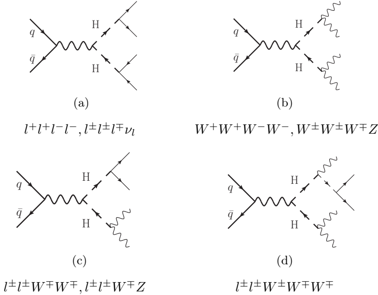
Fig. 1. (a), (b), (c): Doubly-charged scalar pair ( H^{++}H^{--} ) and associated ( H^{\pm\pm}H^{\mp} ) production diagrams. (d): Associated production with a triply-charged scalar ( H^{\pm\pm\pm}H^{\mp\mp\mp} ) when the multiplet also has a component with charge |Q| = 3 .
