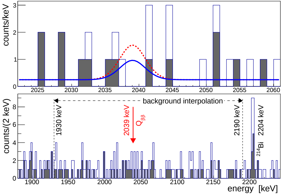
Fig. 1. The GERDA Phase I energy spectrum from all enriched detectors with and without PSD shown by the filled and open histograms, respectively. The lower panel shows the region used for the background interpolation. The spectrum in the upper plot is zoomed to Q_{\beta\beta} and it was superimposed with the expectations (with PSD selection) based on the central value of [5] ( T_{1/2}^{0\nu} = 1.19 \times 10^{25} yr — dashed/red) and with the 90% upper limit derived by GERDA ( T_{1/2}^{0\nu} = 2.10 \times 10^{25} yr).
