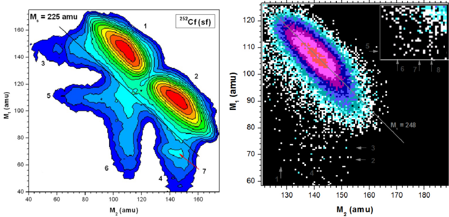
Fig. 5. Left part: The M_1 – M_2 mass correlation for two fission fragments in coincidence in two FOBOS detectors, see Fig. 4. The two binary fission mass peaks have their maximum at a sum M_s = 250 , well above the line showing the total mass of M_s = 232 , which separates the main binary yield. The missing mass bump in arm1 is marked by an arrow (masses M_1 = 68 and M_2 = 144 ), it is absent in arm2. Right-hand side: measurements with the COMETA detectors (Fig. 3) in Ex4. Below the fission bump (in arm1), of the binary fission of Cf in the correlation ( M_1, M_2 ), we observe two horizontal lines (marked by arrows), which we attribute to Ni (or Cr) isotopes, see Fig. 3.
