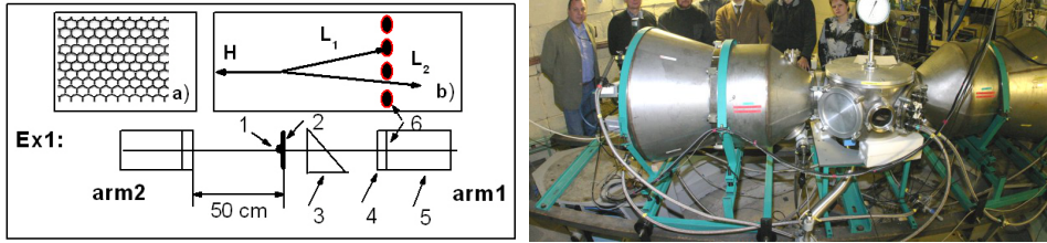
Fig. 4. Scheme of (Ex1) for coincidence arrangement for the measurements of two fragments of the fission decay of ^{252}\text{Cf} , with two arms (arm1, and arm2). Here: 1 — Cf source, 2 — source backing, 3 — micro-channel plate (MCP) based timing “start” detector, 4–6 FOBOS detectors, Bragg-ionisation chambers, 4 — position sensitive avalanche counter (PSAC) as “stop” detector, 5 — ionization chamber (BIC) with the supporting mesh, 6 — the mesh of the entrance window. The front view of the mesh is shown in the insert (a), an enlarged mesh section is presented in the insert (b). After passage of the two fragments through the source backing, two light fragments L_1 and L_2 , are obtained with a small angle divergence due to multiple scattering. In (b) we show that one of the fragments ( L_1 ) can be lost hitting the metal structure of the mesh, while the fragment L_2 reaches the detectors. The source backing (2) causes the mentioned angular dispersion in the direction towards the right arm1. On the right-hand side, a photograph of the FOBOS-modules is shown.
