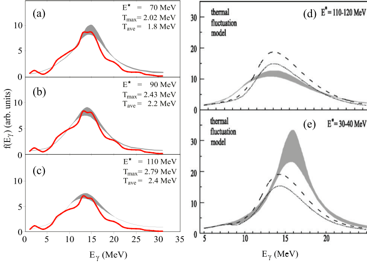
Fig. 2. Experimental (shaded areas) and theoretical shapes for GDR in ^{120}\text{Sn} generated by the CASCADE code at various excitation energies. (a)–(c) predictions generated by using the PDM strength functions. (d) and (e) [9] dotted and dashed lines are generated by using the TSFM strength functions, exhausting 80% and 100% TRK sum rule, respectively.
