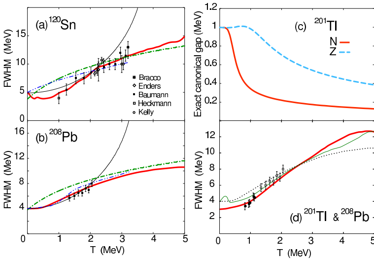
Fig. 1. GDR widths for ^{120}\text{Sn} (a) and ^{208}\text{Pb} (b) predicted by the PDM (thick solid), pTSFM (dot-dashed), AM (double dot-dashed), and FLDM (thin solid) as functions of T in comparison with experimental data in tin and lead regions. (c) Exact canonical neutron ( N ) and proton ( Z ) pairing gaps for ^{201}\text{Tl} as functions of T . (d) GDR width for ^{201}\text{Tl} obtained within the PDM as a function of T (thick solid) including the exact canonical gaps in (c) in comparison with the experimental data for ^{201}\text{Tl} (black circles) and ^{208}\text{Pb} (open boxes). The thin solid line is the PDM result without the effect of thermal pairing. The dotted line is the PDM result for ^{208}\text{Pb} (the same as the thick solid line in (b)).
