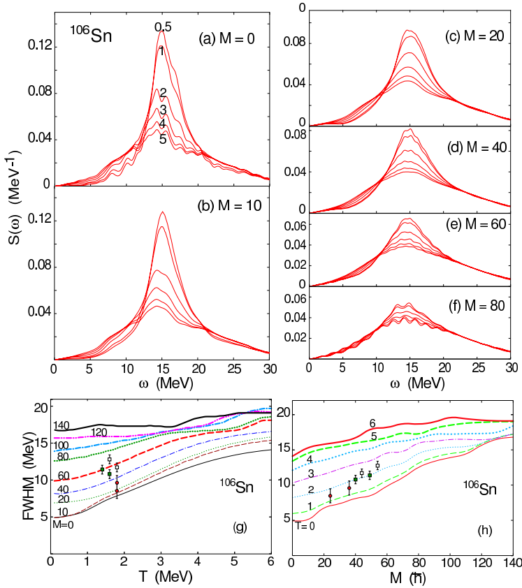
Fig. 3. (a)–(f) GDR strength functions for ^{106}\text{Sn} at T = 0.5, 1, 2, 3, 4 , and 5 MeV as shown at the curves and M = 0, 10, 20, 40, 60 , and 80\hbar as shown in the panels. (g) FWHM of GDR for ^{106}\text{Sn} as a function of T at several values of M (in \hbar ) shown at the curves, (h) FWHM of GDR for ^{106}\text{Sn} as a function of M at several values of T (in MeV) shown at the curves. The experimental data for GDR in ^{106}\text{Sn} (solid circles), ^{109,110}\text{Sn} (open boxes) are adapted from Refs. [19, 20].
