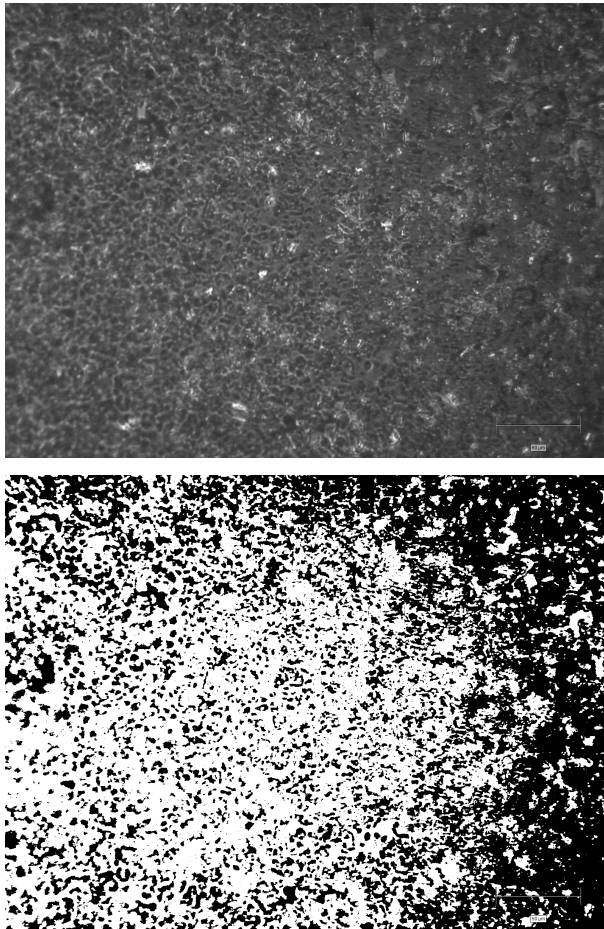
Fig. 1. Typical structure for ethylocellulose membrane with magnetic powder MQP-16 ( 5\text{ }\mu\text{m} ) (top) from optical microscopy, (bottom) digitized image, as required for the fractal analyses, i.e. grey-level threshold techniques provide binary image.
