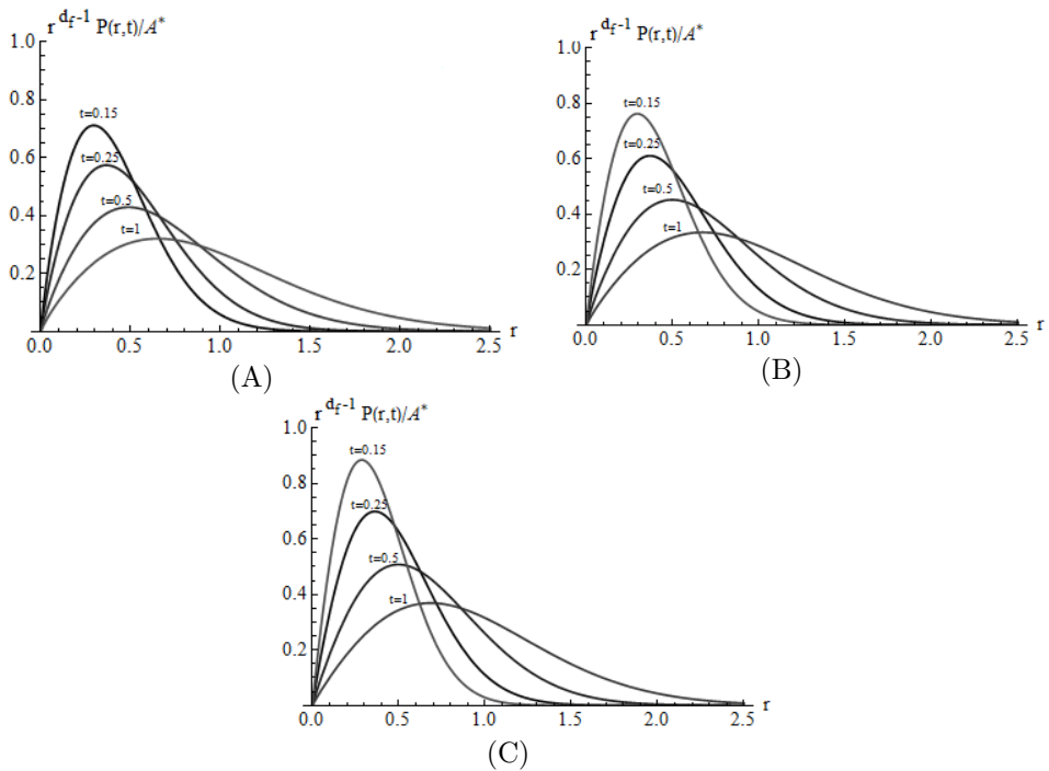
Fig. 4. Probability density at times t = 0.15, 0.25, 0.5, 1 for membranes with dispersed magnetic powder (A) MQP-16 (< 5 \mu\text{m} ), d_f = 1.86 , d_w = 2.38 (B) MQP-16 (5-20 \mu\text{m} ) d_f = 1.90 , d_w = 2.30 (C) MQP-16 (> 20 \mu\text{m} ) d_f = 1.93 , d_w = 2.17 .
