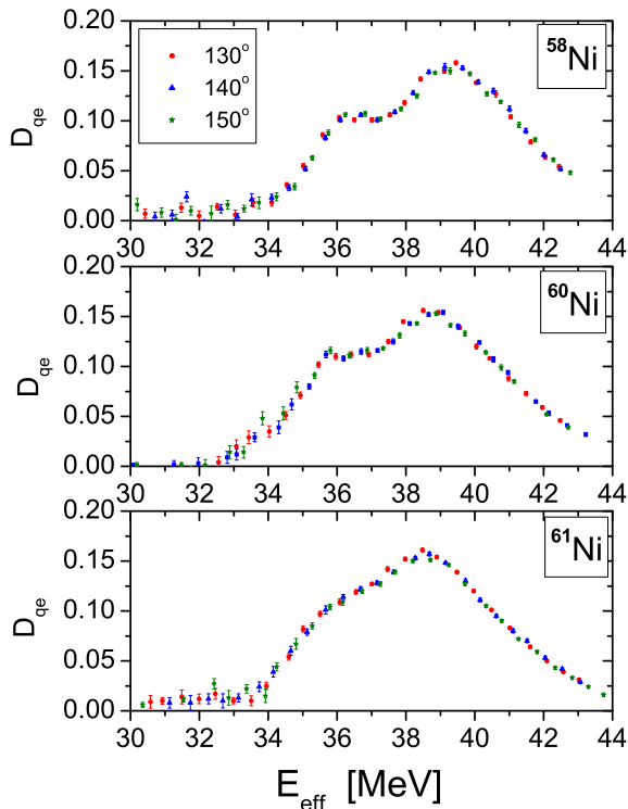
Fig. 4. Barrier height distributions for the ^{20}\text{Ne} + ^{58,60,61}\text{Ni} systems.
