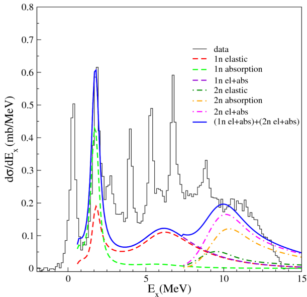
Fig. 1. (Colour on-line) Inclusive energy spectrum of the reaction ^9\text{Be}(^{18}\text{O}, ^{16}\text{O})^{11}\text{Be} at 3^\circ < \theta_{\text{lab}} < 10^\circ obtained after the subtraction of the background due to the contaminants in the target. Theoretical calculations of various break-up components (see the text): the one- and two-neutron elastic break-up; the one- and two-neutron absorption term; the sum of the one- and two-neutron elastic and absorption terms; the sum of all the contributions.
