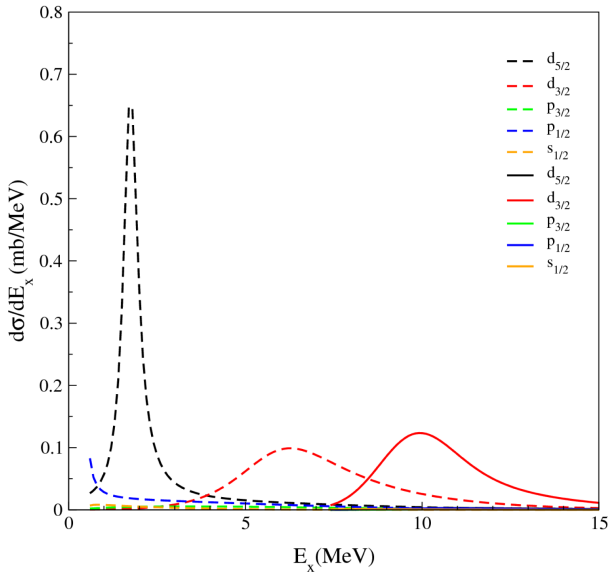
Fig. 2. (Colour on-line) Dominant contributions to the partial wave decomposition of the theoretical energy spectrum. The legend indicates the single particle angular momentum of each individual strength distribution. The lines starting at E_x = 0.501 MeV refer to the ^{10}\text{Be} + n system, while those starting at 7.313 MeV to the ^9\text{Be} + n + n one (see the text).
