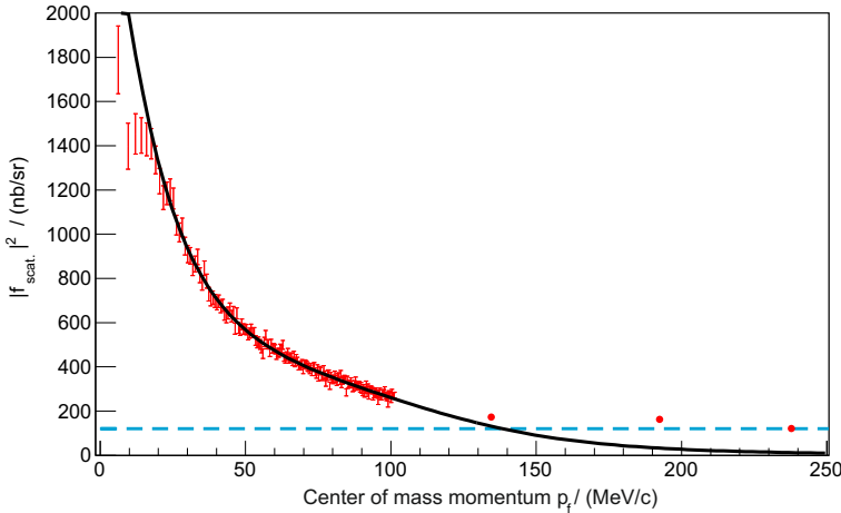
Fig. 2. Scattering amplitude squared extracted from the unpolarised data obtained at ANKE as function of the \eta c.m. momentum. The solid line shows the result of a fit to the near-threshold data, whereas the dashed line shows an expectation according to pure phase space behaviour, arbitrarily fixed to the highest energy data point.
