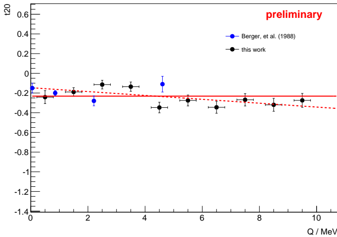
Fig. 3. Energy dependence of the deuteron tensor analysing power t_{20} close to the production threshold. The solid line corresponds to a fit to the data assuming a constant analysing power while the fit indicated by the dashed line allows for a linear.
