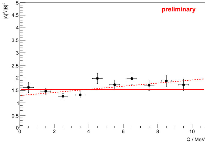
Fig. 4. Ratio of the squared amplitudes |A|^2/|B|^2 as function of the excess energy. The solid and dashed lines correspond to a constant fit and a first order polynomial fit, respectively.
