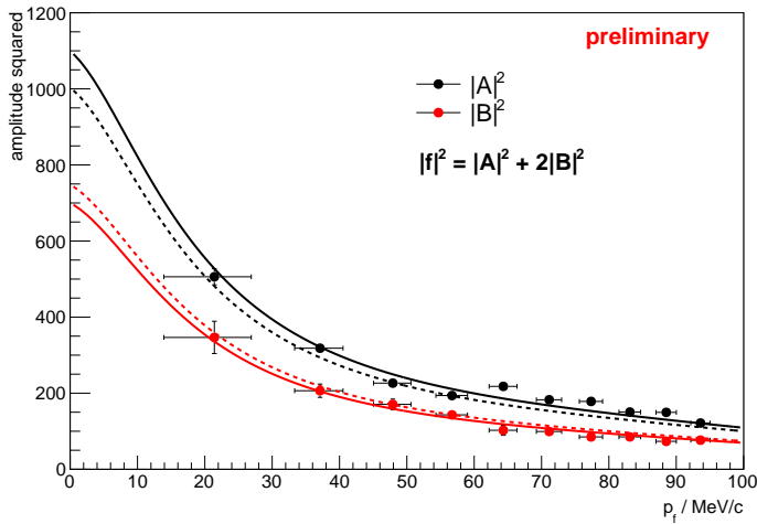
Fig. 5. Energy dependence of the amplitudes |A|^2 and |B|^2 as function of the final state momentum p_f . The solid lines have been obtained by the assumption of a constant ratio |A|^2/|B|^2 close to threshold and using the squared amplitudes |f_{\text{scat}}|^2 from unpolarised data.
