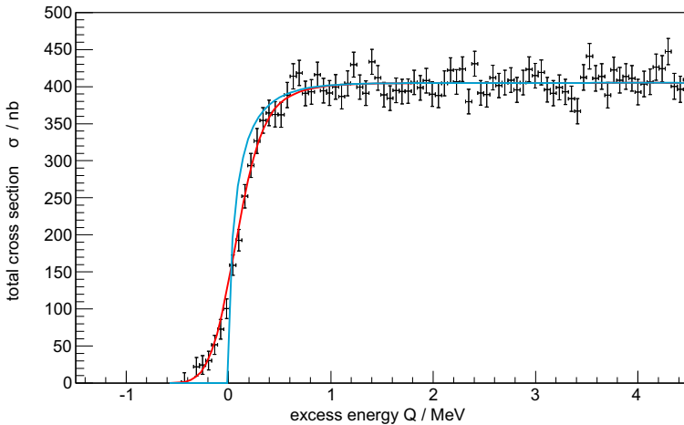
Fig. 1. Total cross sections for the dp \rightarrow {}^3\text{He} \eta reaction in the very near threshold region, i.e. for Q < 4.5 MeV. The solid line starting in the sub-threshold region corresponds to a fit to the results considering a strong final state interaction as well as the finite COSY beam momentum width, while the other one is the result to be expected without the 180 keV smearing in Q .
