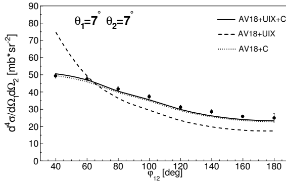
Fig. 1. Differential, integrated over energy, cross-section values presented as a function of the relative azimuthal angle \varphi_{12} , for a given \theta_1, \theta_2 combination. The data are compared with the calculations indicated in the legend.
