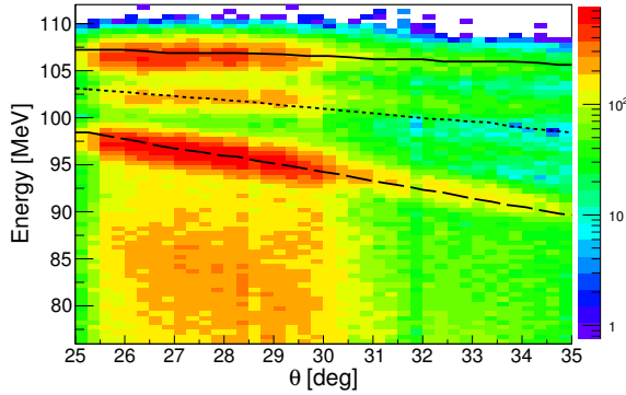
Fig. 2. Kinematical relation for protons scattered from a \text{C}_2\text{D}_4 target. Presented data were registered in one E -slab. The lines represent the kinematics calculated for the following elastic scattering processes: p + ^{12}\text{C} (solid), p + ^4\text{He} (dotted), p + d (dashed).
