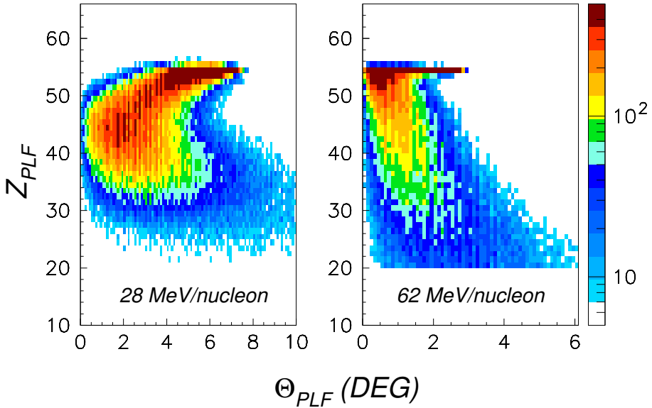
Fig. 3. (Color online) Logarithmic contour plots of the PLF charge ( Z_{\text{PLF}} ) as a function detected PLF angle ( \Theta_{\text{PLF}} ) in LAB system representation, for bombarding energy 28 and 62 MeV/nucleon, as obtained from QMD simulation with deexcitation phase simulated by equilibrium-statistical decay code GEMINI.
